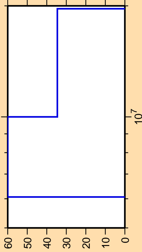
\Delta\sigma/\sigma vs. E for ^{232}\text{Np}(n,d)
