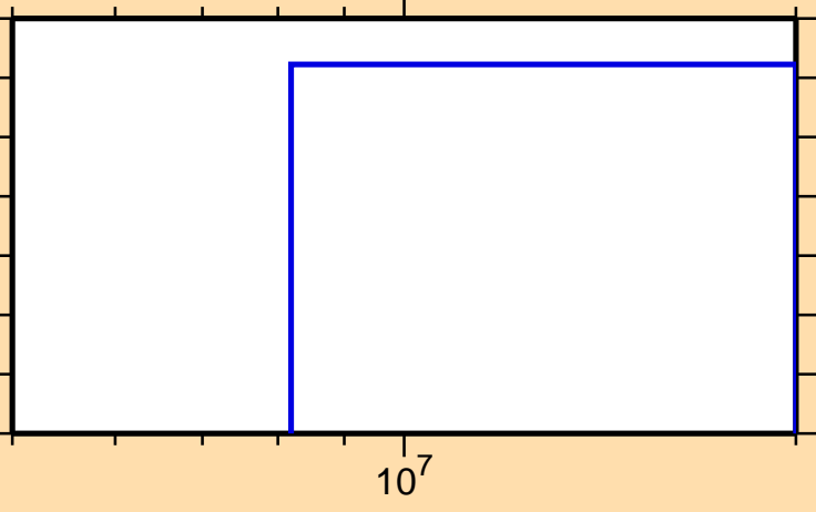
\sigma vs. E for ^{232}\text{Np}(n,nd)
