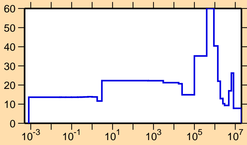
\Delta\sigma/\sigma vs. E for ^{232}\text{Np}(n,el.)
