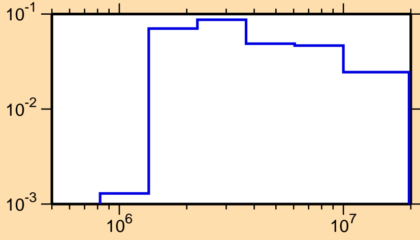
\sigma vs. E for ^{233}\text{Np}(n,n\text{cont.})
