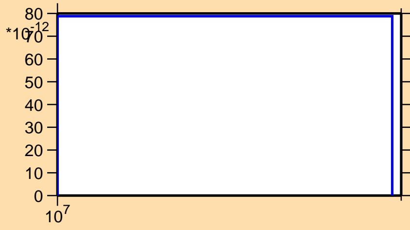
\sigma vs. E for ^{233}\text{Np}(n,\text{He}3)
