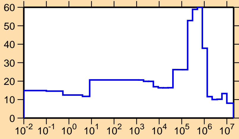
\Delta\sigma/\sigma vs. E for ^{233}\text{Np}(n,el.)
