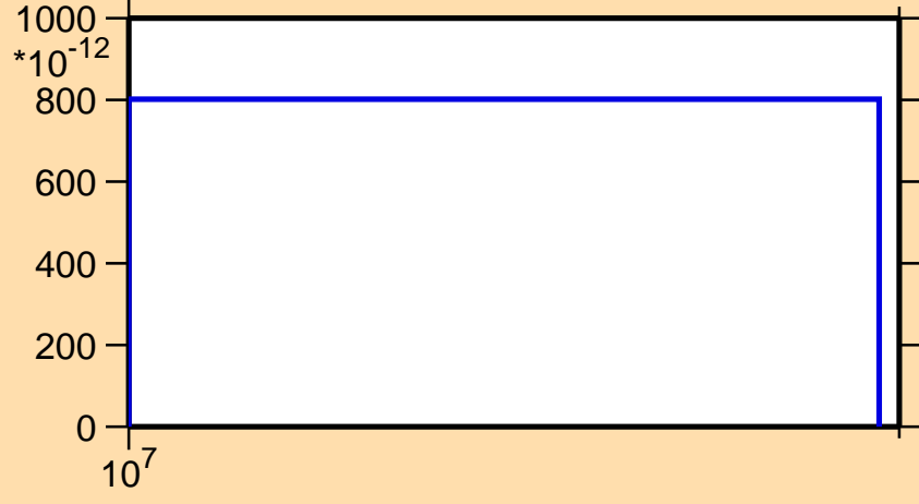
\sigma vs. E for ^{233}\text{Np}(n,nd)
