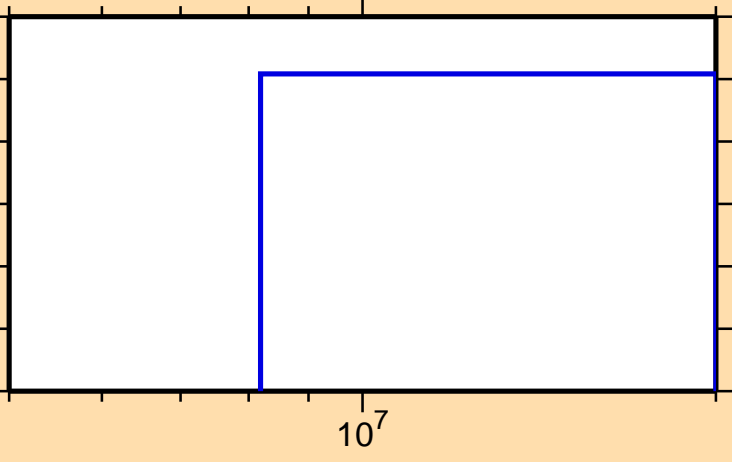
\sigma vs. E for ^{233}\text{Np}(n,t)
