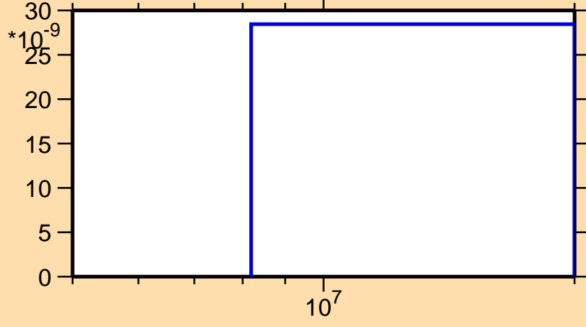
\sigma vs. E for ^{233}\text{Np}(n,nt)
