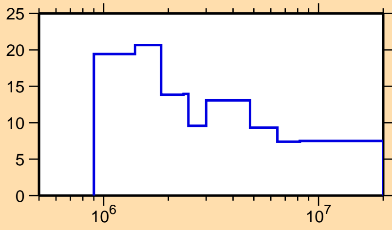
\Delta\sigma/\sigma vs. E for ^{233}\text{Np}(n,\text{nonel.})
