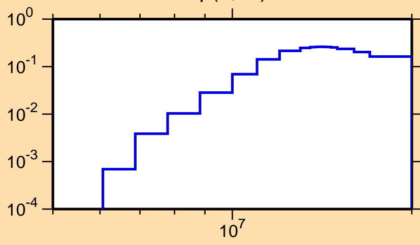
\sigma vs. E for ^{234}\text{Np}(n,2n)
