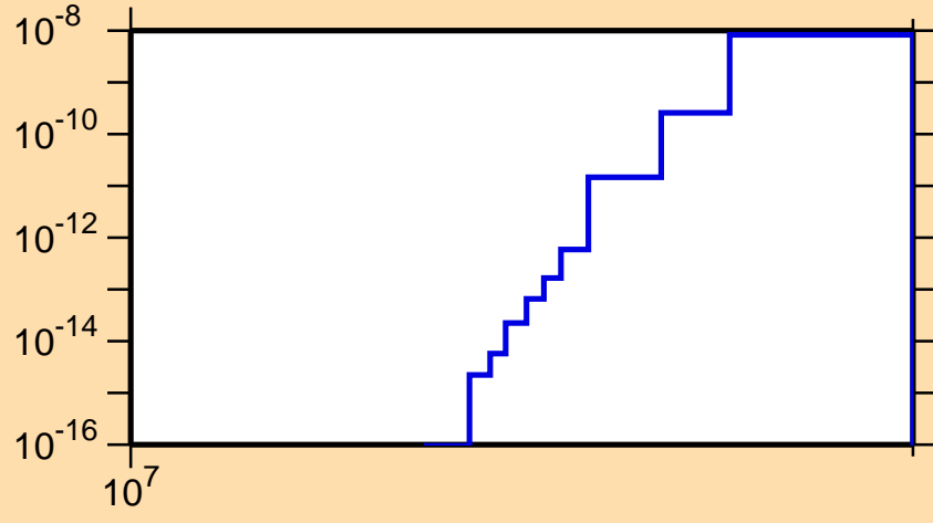
\sigma vs. E for ^{234}\text{Np}(n,nt)
