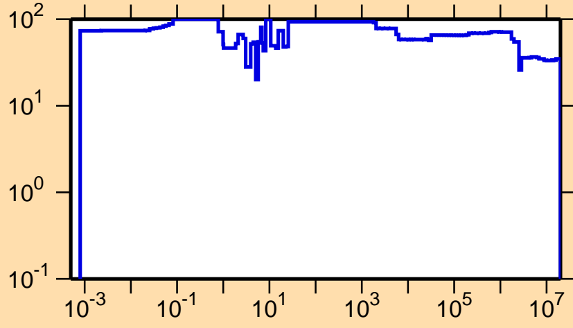
\Delta\sigma/\sigma vs. E for ^{234}\text{Np}(n,\gamma)
