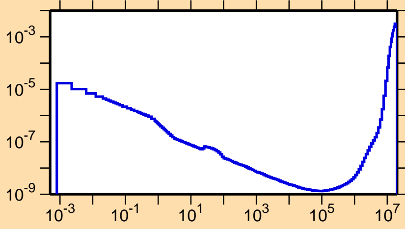
\sigma vs. E for ^{234}\text{Np}(n,\alpha)
