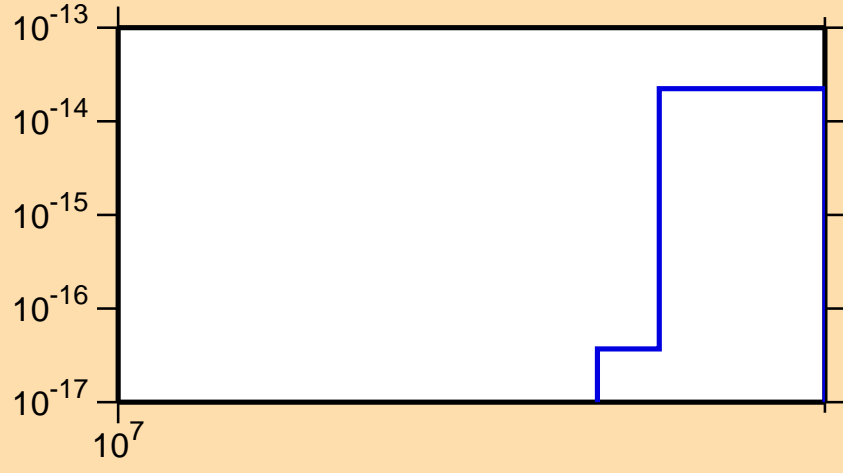
\sigma vs. E for ^{234}\text{Np} (mt 34)
