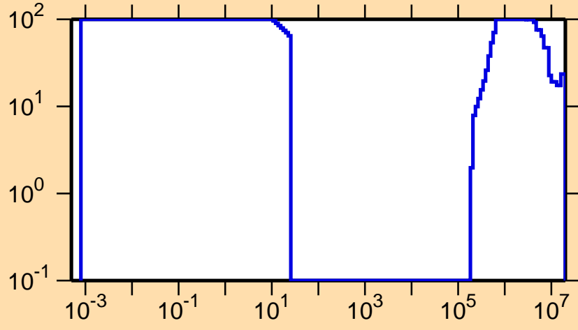
\Delta\sigma/\sigma vs. E for ^{234}\text{Np}(n,p)
