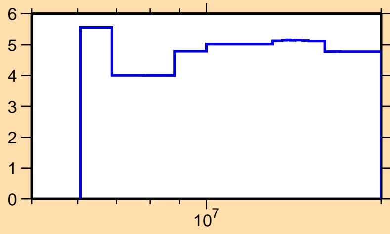
\Delta\sigma/\sigma vs. E for ^{234}\text{Np}(n,\text{nonel.})
