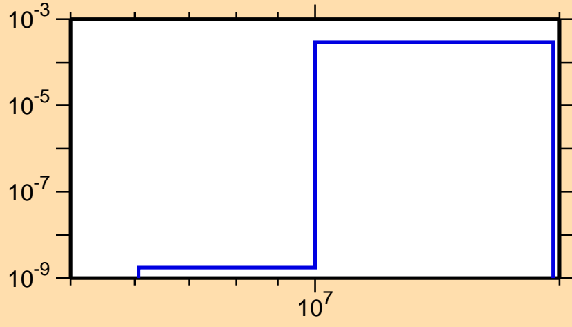
\sigma vs. E for ^{234}\text{Np}(n,np)
