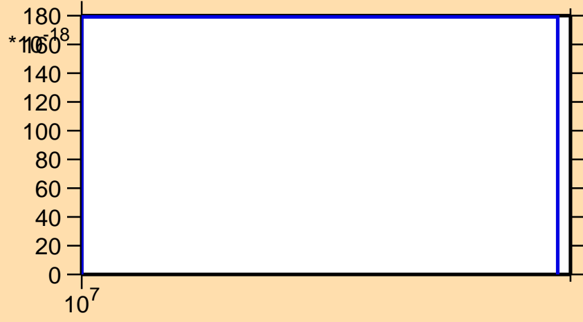
\sigma vs. E for ^{234}\text{Np} (mt 34)
