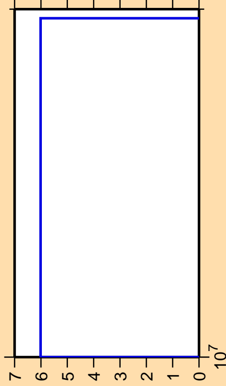
\Delta\sigma/\sigma vs. E for ^{234}\text{Np}(n,p\alpha)
