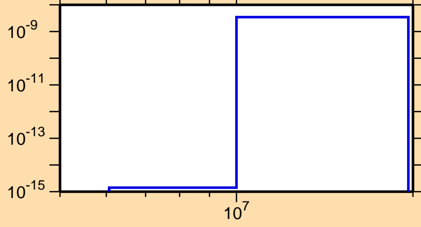
\sigma vs. E for ^{234}\text{Np}(n,2n\alpha)
