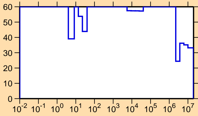
\Delta\sigma/\sigma vs. E for ^{234}\text{Np}(n,\gamma)
