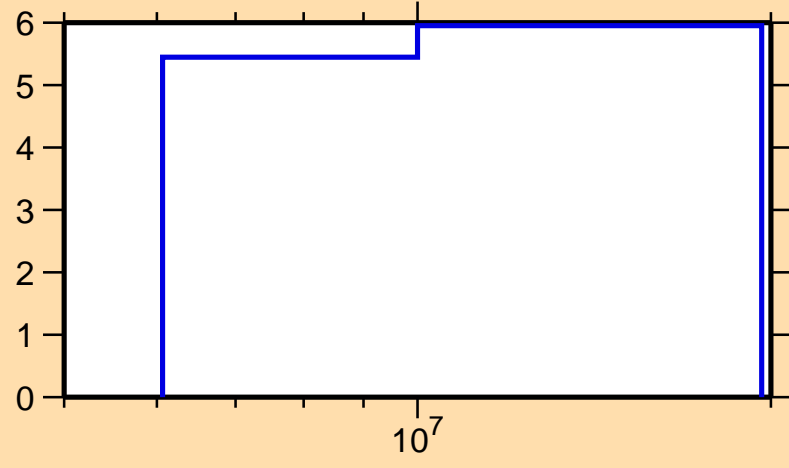
\Delta\sigma/\sigma vs. E for ^{234}\text{Np}(n,\text{tot.})
