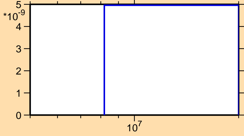
\sigma vs. E for ^{234}\text{Np}(n,nd)
