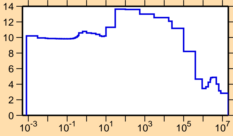
\sigma vs. E for ^{234}\text{Np}(n,\text{el.})
