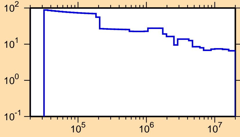
\Delta\sigma/\sigma vs. E for ^{2335}\text{Np}(n,\text{nonel.})
