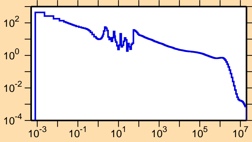
\sigma vs. E for ^{235}\text{Np}(n,\gamma)
