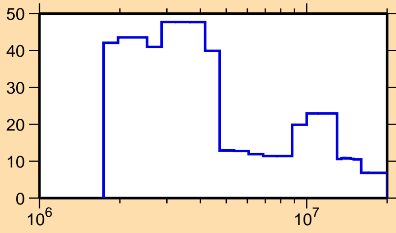
\Delta\sigma/\sigma vs. E for ^{235}\text{Np}(n,f)
