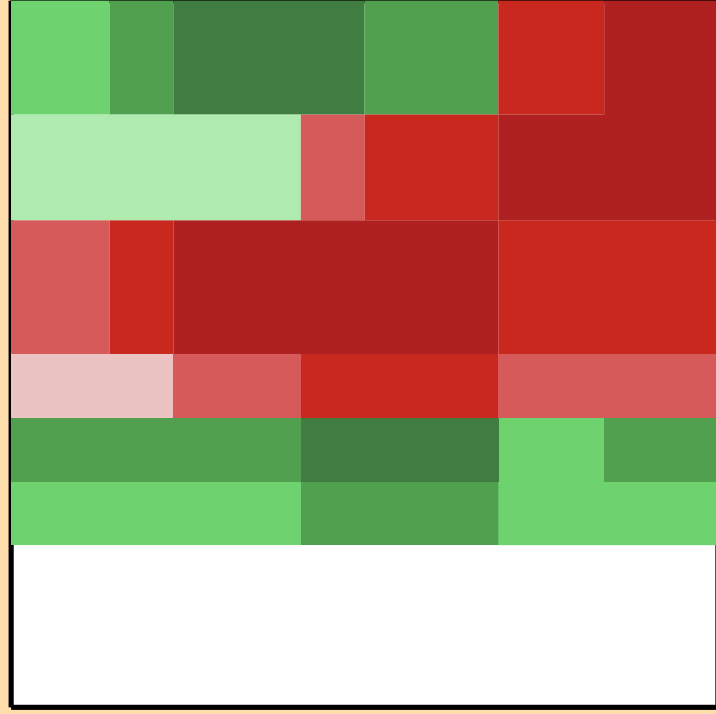
\Delta\sigma/\sigma vs. E for ^{235}\text{Np}(n,\text{el.})
