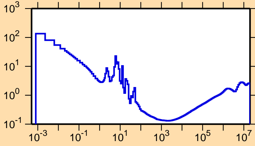
\sigma vs. E for ^{235}\text{Np}(n,f)
