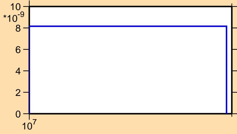
\sigma vs. E for ^{235}\text{Np}(n,nd)
