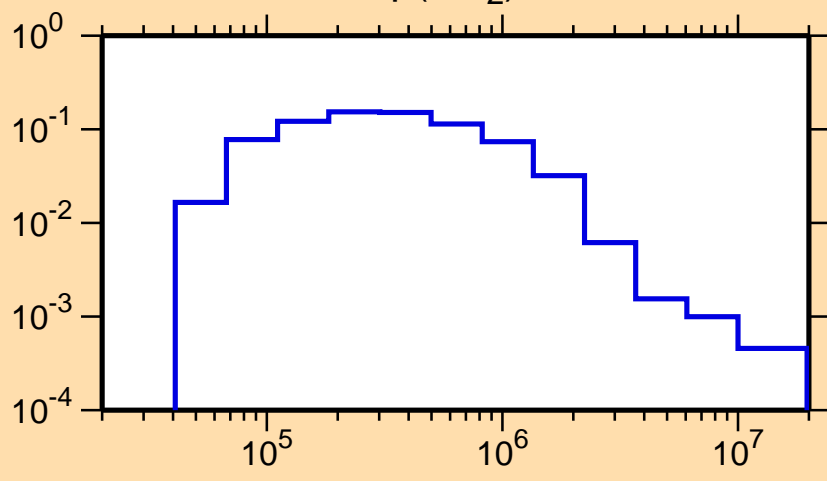
\sigma vs. E for ^{235}\text{Np}(n,n_2)
