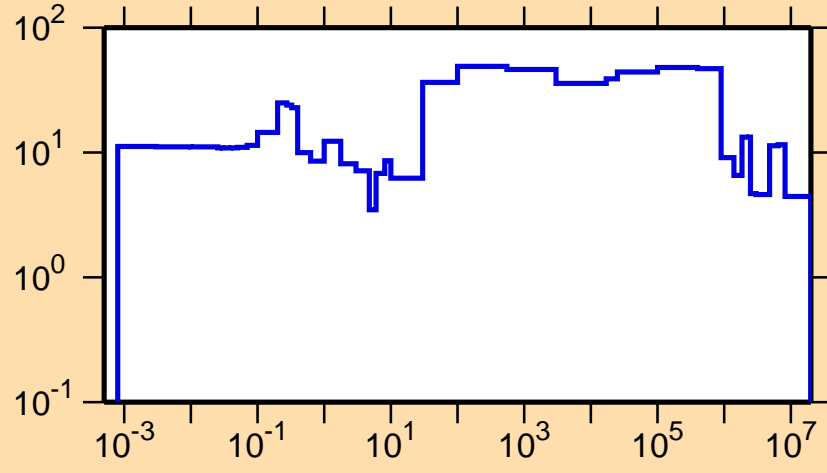
\Delta\sigma/\sigma vs. E for ^{235}\text{Np}(n,tot.)
