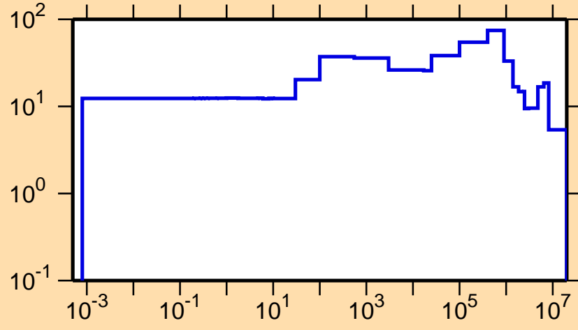
\Delta\sigma/\sigma vs. E for ^{235}\text{Np}(n,el.)
