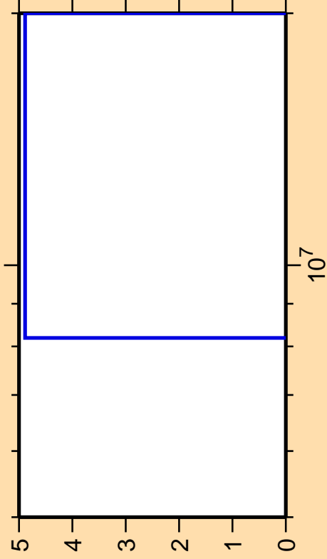
\Delta\sigma/\sigma vs. E for ^{235}\text{Np}(n,\text{He3})
