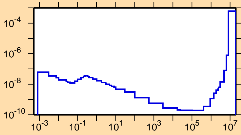
\sigma vs. E for ^{235}\text{Np}(n,\alpha)
