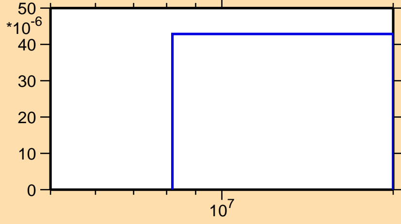
\sigma vs. E for ^{235}\text{Np}(n,t)
