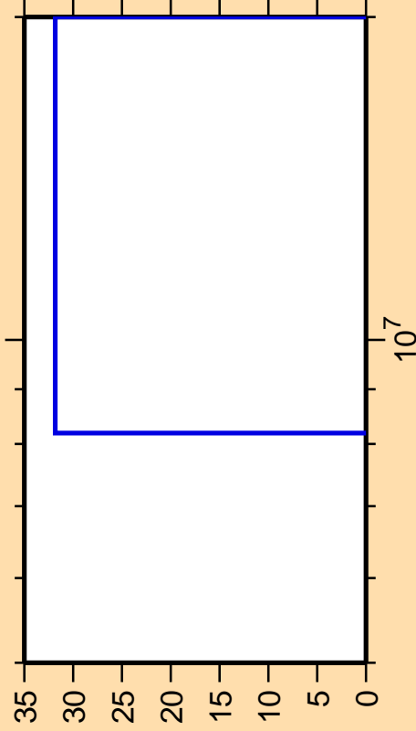
\Delta\sigma/\sigma vs. E for ^{235}\text{Np}(n,t)
