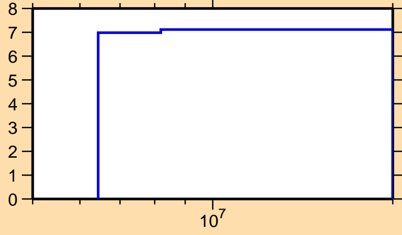
\Delta\sigma/\sigma vs. E for ^{235}\text{Np}(n,\text{nonel.})
