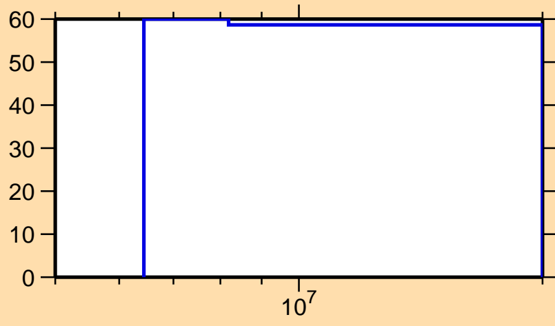
\Delta\sigma/\sigma vs. E for ^{235}\text{Np}(n,2n)
