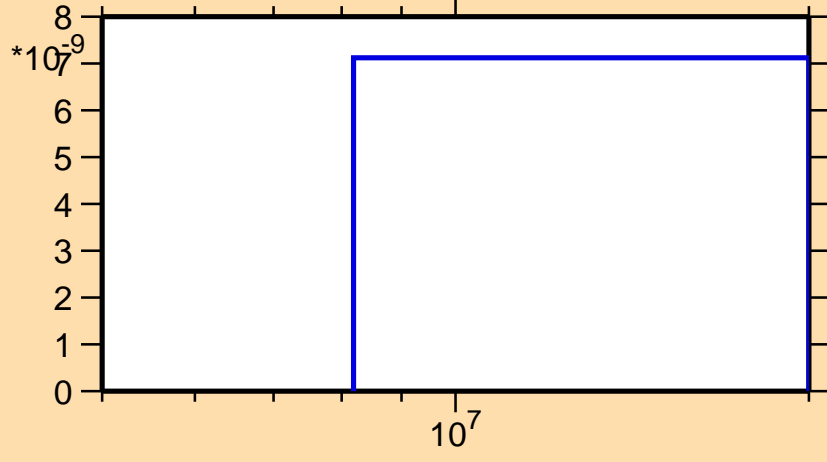
\sigma vs. E for ^{235}\text{Np}(n,nd)
