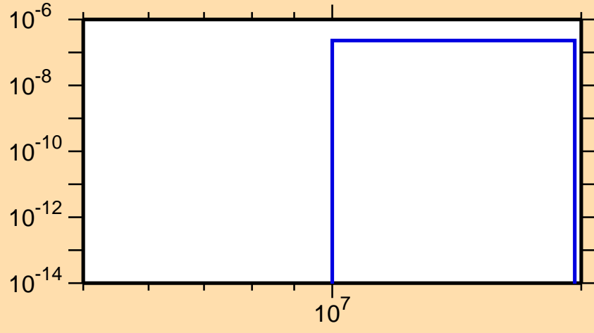
\sigma vs. E for ^{236}\text{Np}(n,\text{nd})
