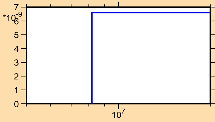
\sigma vs. E for ^{236}\text{Np}(n,2n\alpha)
