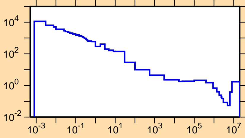
\sigma vs. E for ^{236}\text{Np}(n,f)
