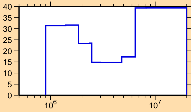
\Delta\sigma/\sigma vs. E for ^{236}\text{Np}(n,ncont.)
