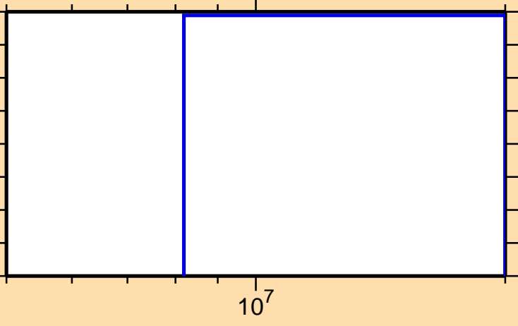
\sigma vs. E for ^{236}\text{Np}(n,nt)
