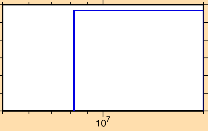
\sigma vs. E for ^{236}\text{Np}(n,2np)
