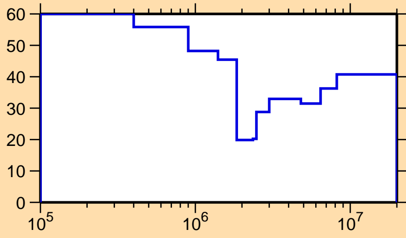
\Delta\sigma/\sigma vs. E for ^{236}\text{Np}(n,n_1)
