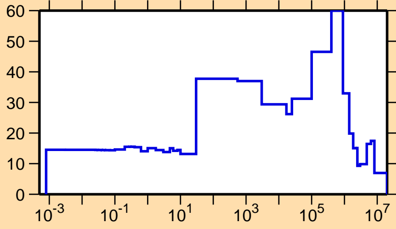
\Delta\sigma/\sigma vs. E for ^{236}\text{Np}(n,el.)
