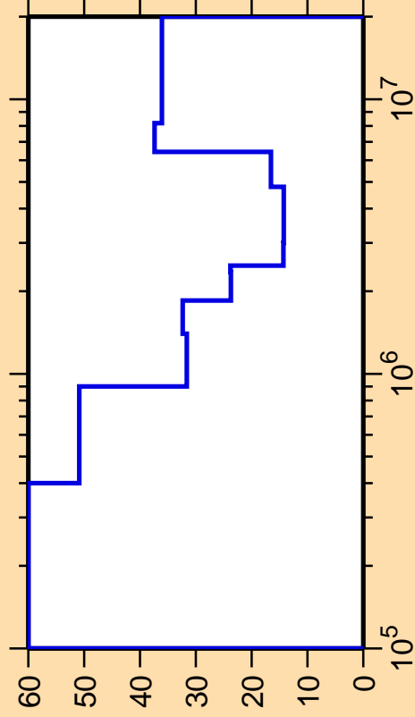
\Delta\sigma/\sigma vs. E for ^{236}\text{Np}(n,\text{inel.})
