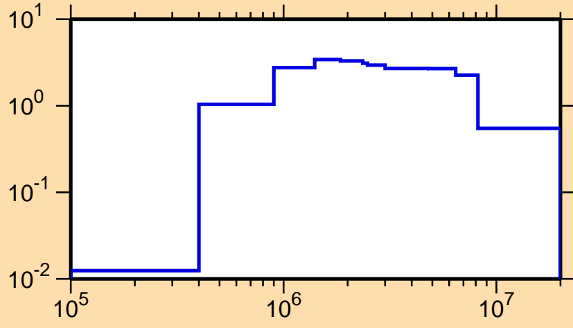
\sigma vs. E for ^{236}\text{Np}(n,\text{inel.})
