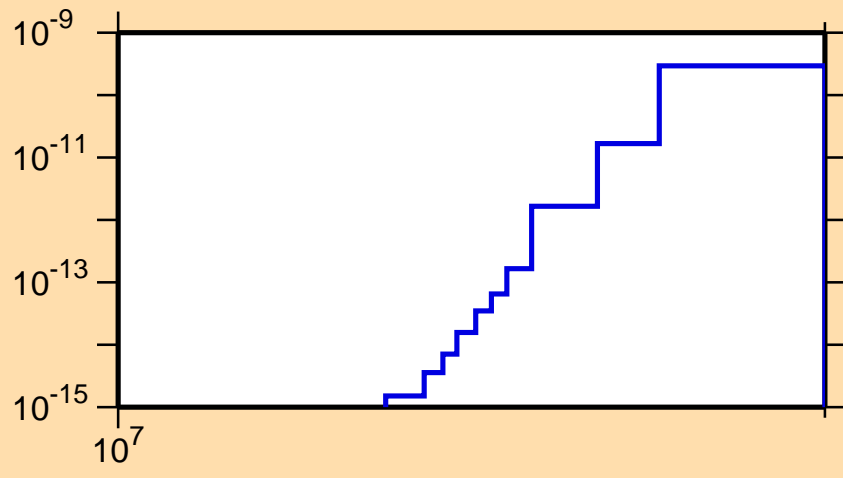
\sigma vs. E for ^{236}\text{Np}(n,\text{He3})
