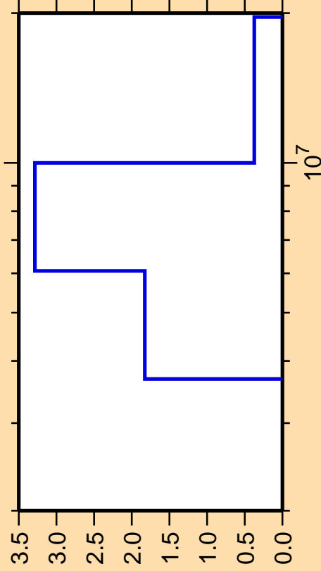
\Delta\sigma/\sigma vs. E for ^{237}\text{Np}(n,n\alpha)
