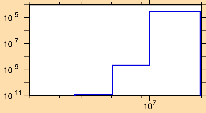
\sigma vs. E for ^{237}\text{Np}(n,n\alpha)
