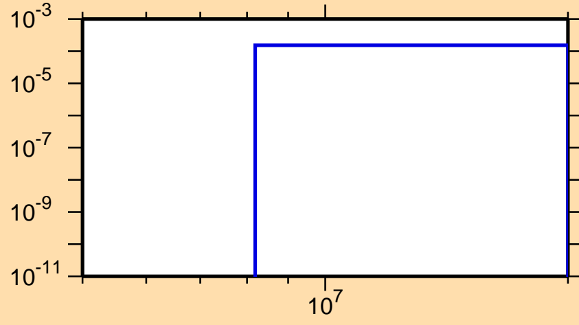
\sigma vs. E for ^{237}\text{Np}(n,d)
