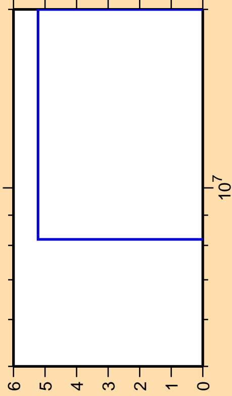
\Delta\sigma/\sigma vs. E for ^{237}\text{Np}(n,nt)
