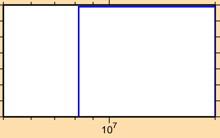
\sigma vs. E for ^{237}\text{Np}(n,np)
