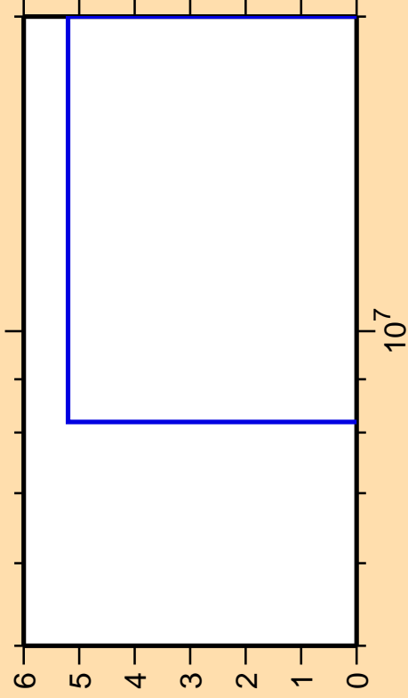
\Delta\sigma/\sigma vs. E for ^{237}\text{Np}(n,nd)
