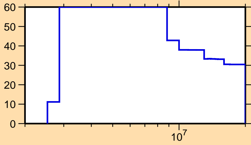
\Delta\sigma/\sigma vs. E for ^{238}\text{Np}(n,p)
