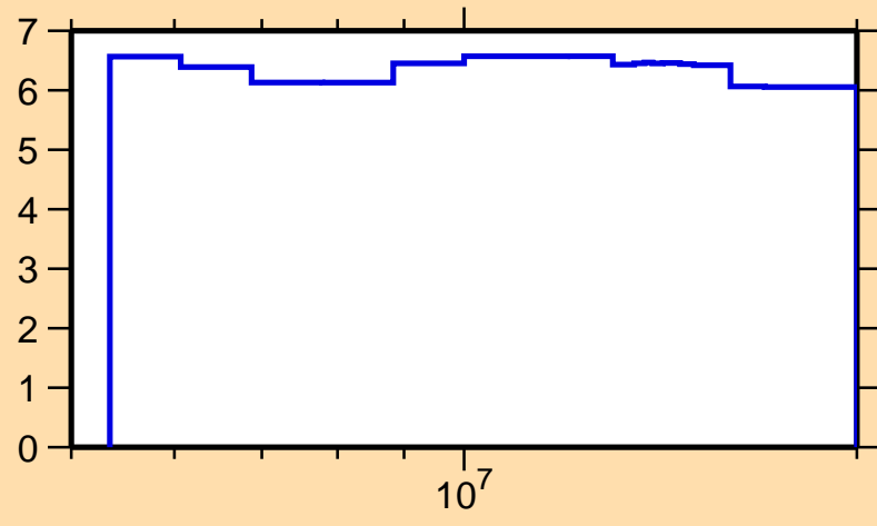
\Delta\sigma/\sigma vs. E for ^{238}\text{Np}(n,\text{nonel.})
