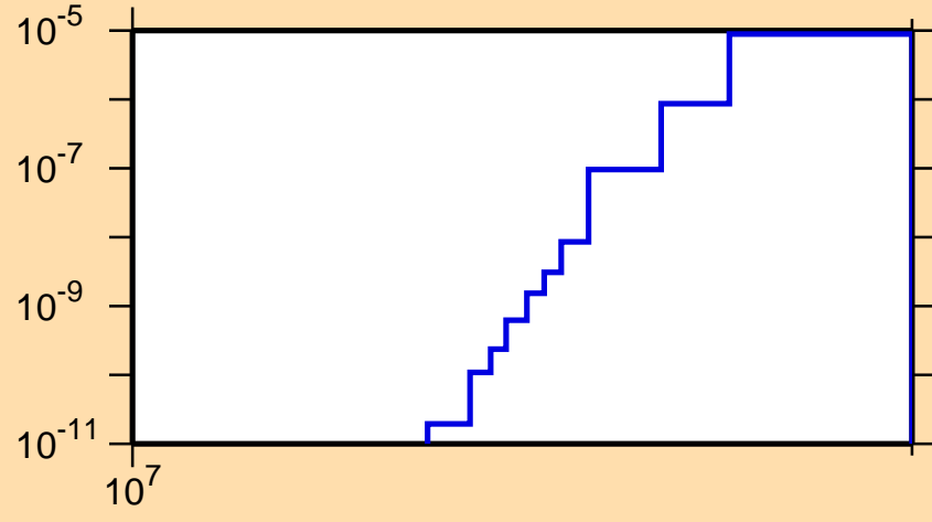
\sigma vs. E for ^{238}\text{Np}(n,nd)
