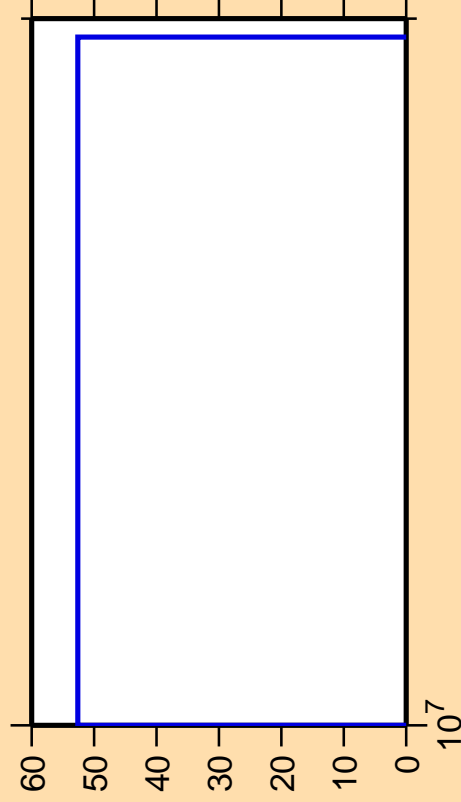
\Delta\sigma/\sigma vs. E for ^{238}\text{Np}(n,\text{nd})
