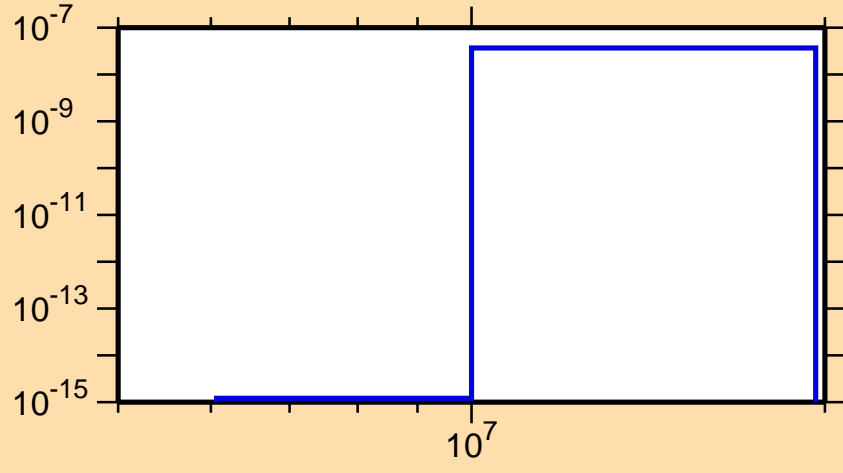
\sigma vs. E for ^{238}\text{Np}(n,2n\alpha)
