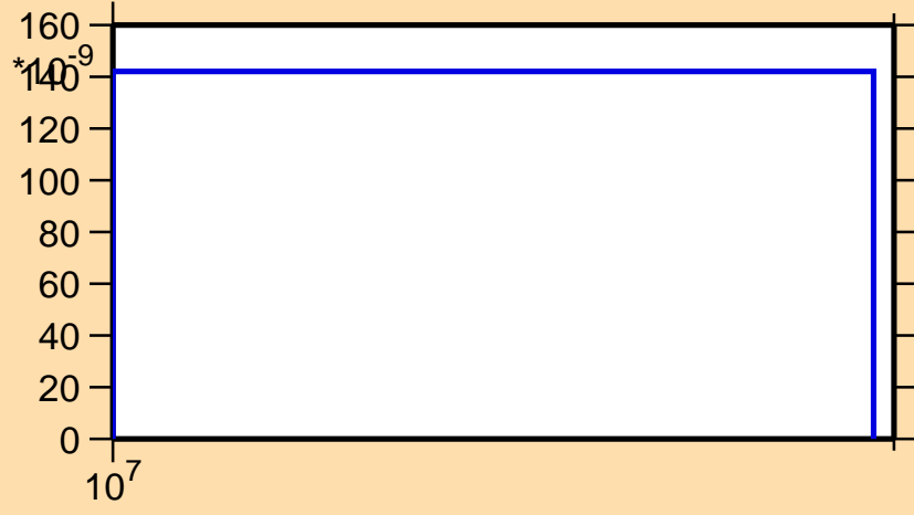
\sigma vs. E for ^{238}\text{Np}(n,\text{nd})
