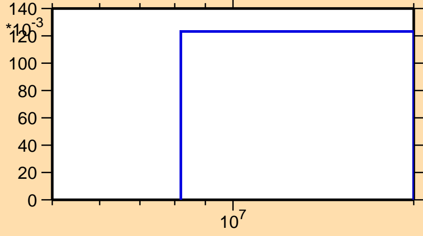
\sigma vs. E for ^{238}\text{Np}(n,3n)
