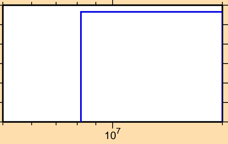
\sigma vs. E for ^{238}\text{Np}(n,2np)
