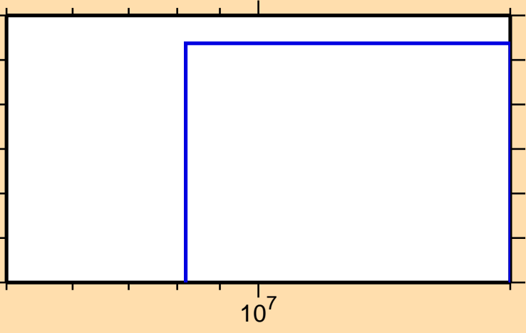
\sigma vs. E for ^{238}\text{Np}(n,nt)
