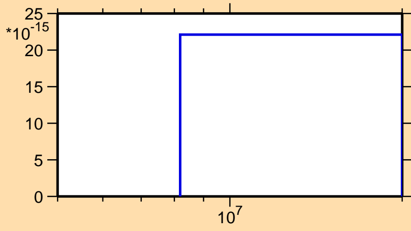
\sigma vs. E for ^{239}\text{Np}(n,\text{He3})
