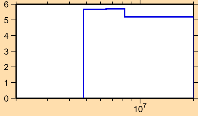
\Delta\sigma/\sigma vs. E for ^{239}\text{Np}(n,\text{nonel.})
