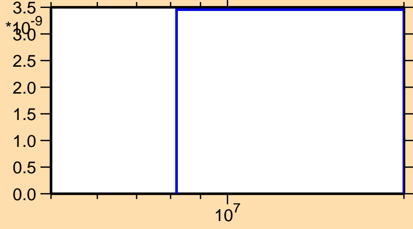
\sigma vs. E for ^{239}\text{Np}(n,2np)
