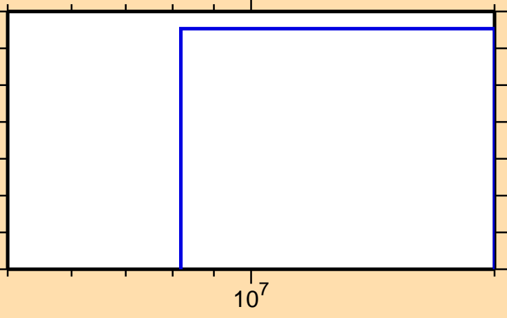
\sigma vs. E for ^{239}\text{Np}(n,t)
