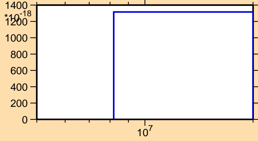
\sigma vs. E for ^{239}\text{Np}(\text{mt } 11)
