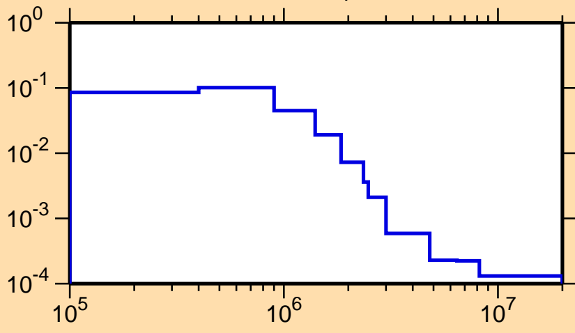
\sigma vs. E for ^{239}\text{Np}(n,n_4)
