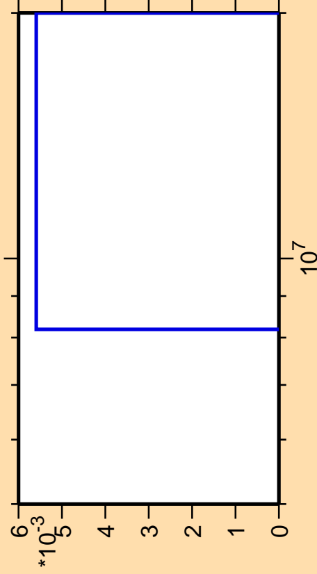
\Delta\sigma/\sigma vs. E for ^{239}\text{Np}(\text{mt } 11)
