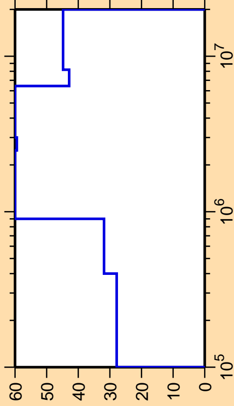
\Delta\sigma/\sigma vs. E for ^{239}\text{Np}(n,n_4)
