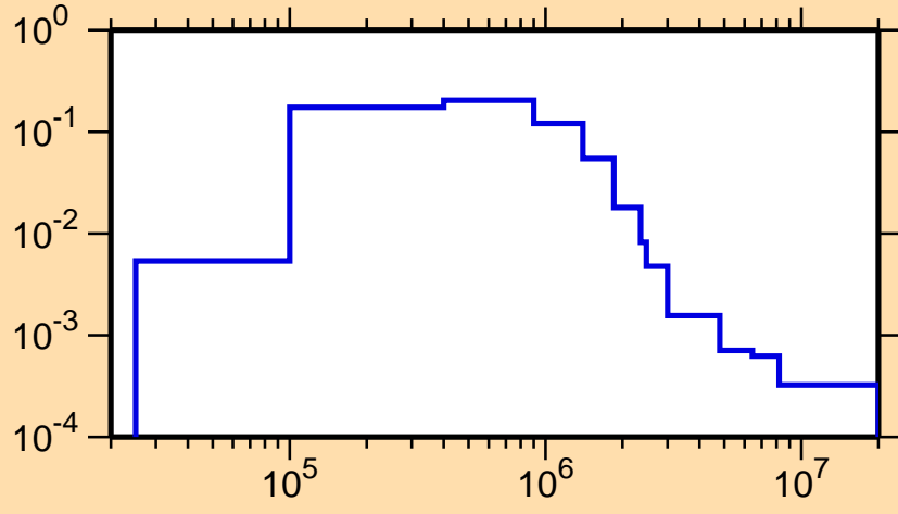
\sigma vs. E for ^{239}\text{Np}(n,n_2)
