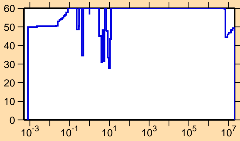
\Delta\sigma/\sigma vs. E for ^{240}\text{Np}(n,\gamma)
