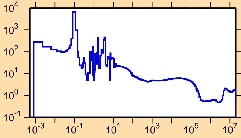
\sigma vs. E for ^{240}\text{Np}(n,f)
