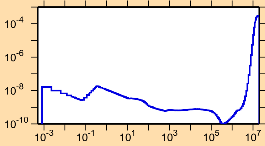
\sigma vs. E for ^{240}\text{Np}(n,\alpha)
