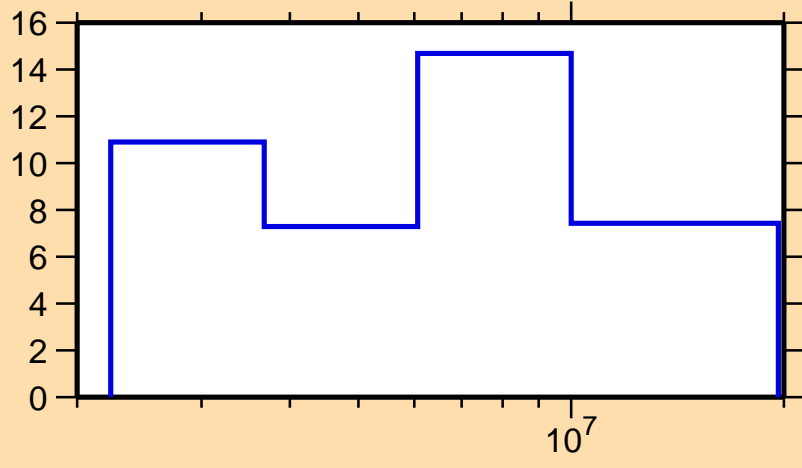
\Delta\sigma/\sigma vs. E for ^{240}\text{Np}(n,el.)
