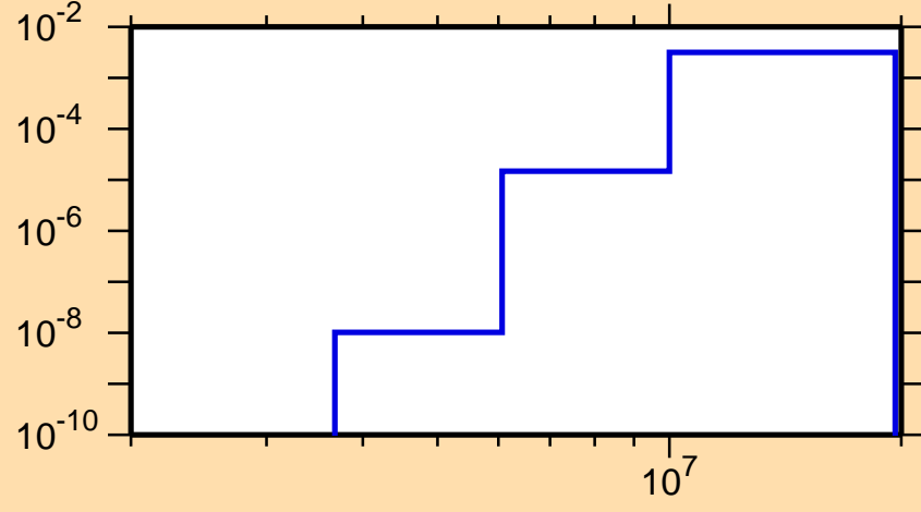
\sigma vs. E for ^{240}\text{Np}(n,p)
