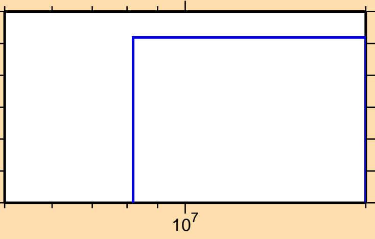
\sigma vs. E for ^{240}\text{Np}(n,\text{He3})
