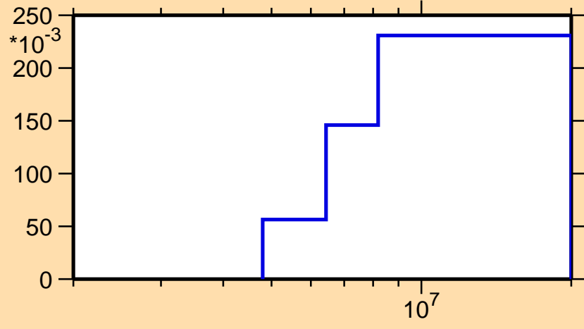
\sigma vs. E for ^{240}\text{Np}(n,2n)
