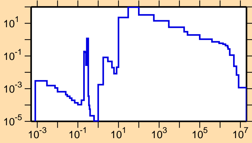
\sigma vs. E for ^{240}\text{Np}(n,\gamma)
