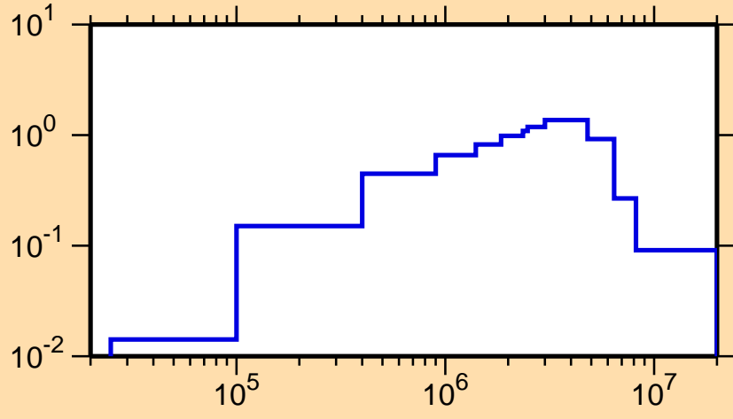
\sigma vs. E for ^{240}\text{Np}(n,n\text{cont.})
