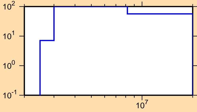
\Delta\sigma/\sigma vs. E for ^{240}\text{Np}(n,p)
