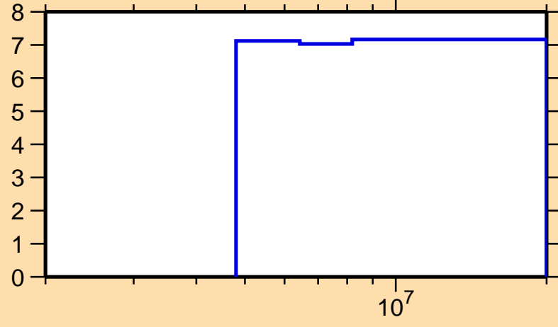
\Delta\sigma/\sigma vs. E for ^{240}\text{Np}(n,\text{nonel.})
