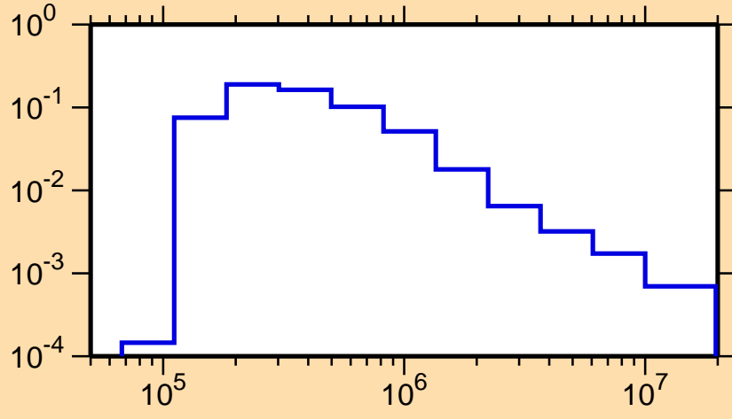
\sigma vs. E for ^{241}\text{Np}(n,n_1)
