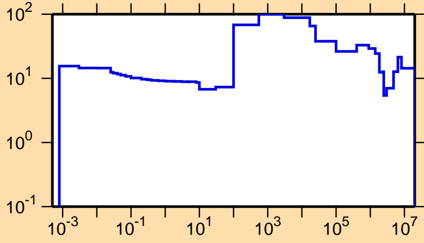
\Delta\sigma/\sigma vs. E for ^{241}\text{Np}(n,tot.)
