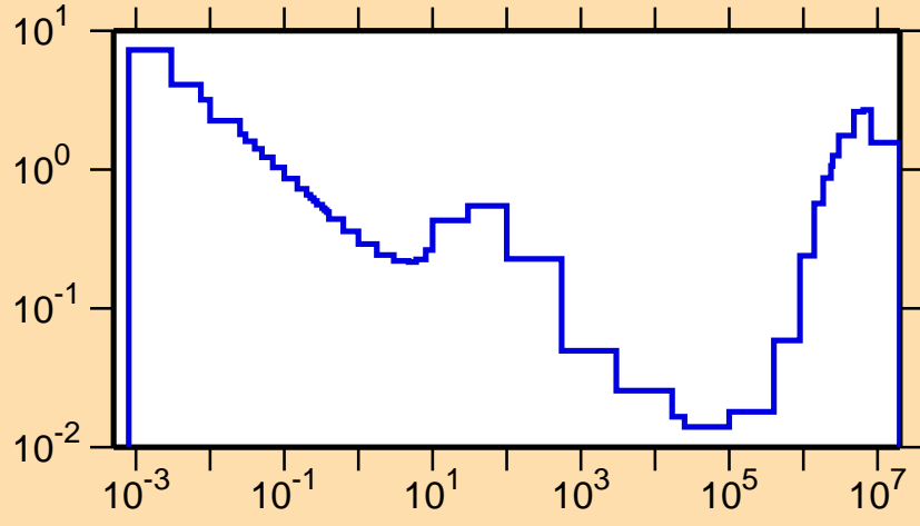
\sigma vs. E for ^{241}\text{Np}(n,f)
