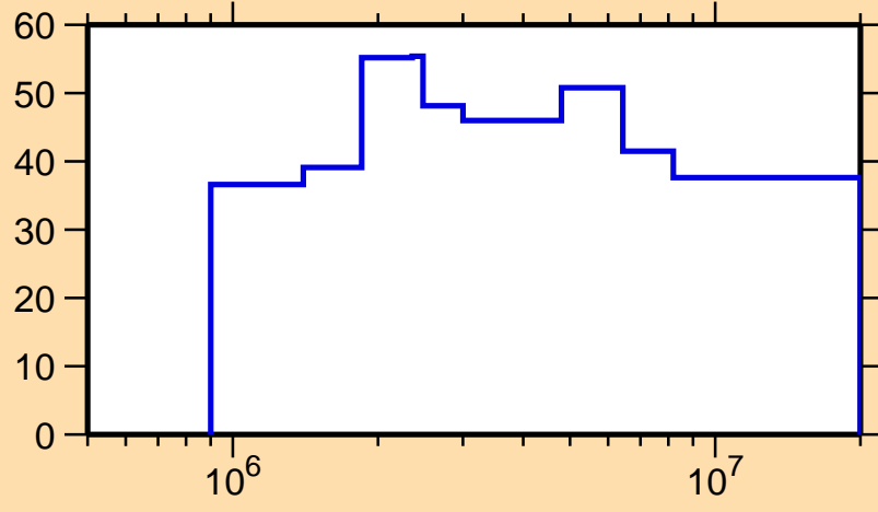
\Delta\sigma/\sigma vs. E for ^{241}\text{Np}(n,n\text{cont.})
