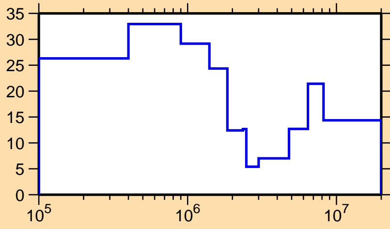
\Delta\sigma/\sigma vs. E for ^{241}\text{Np}(n,\text{tot.})
