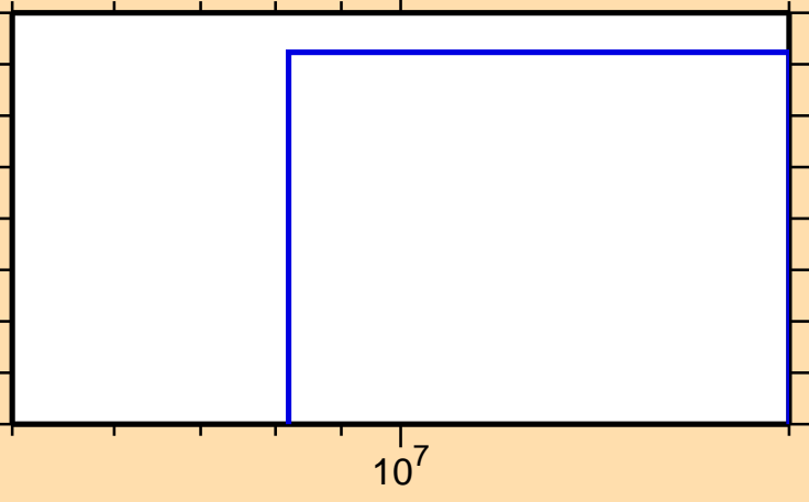
\sigma vs. E for ^{241}\text{Np}(n,nt)
