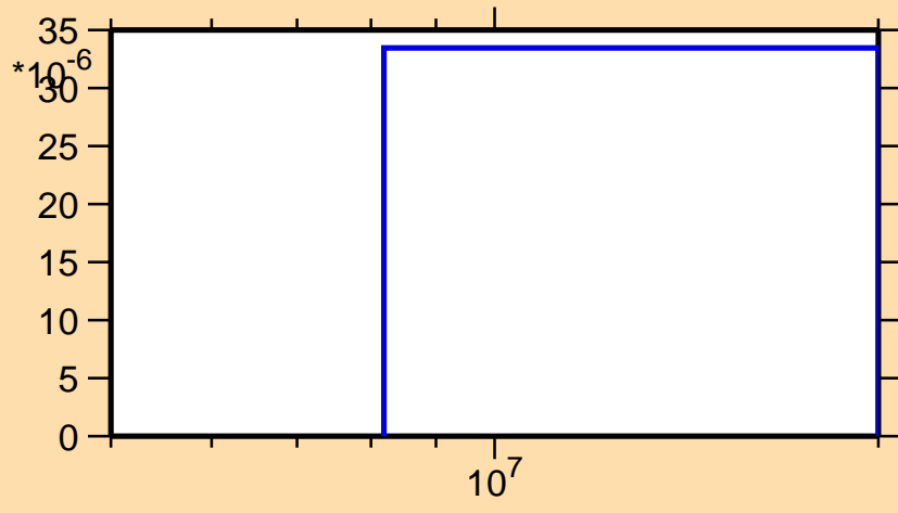
\sigma vs. E for ^{241}\text{Np}(n,np)
