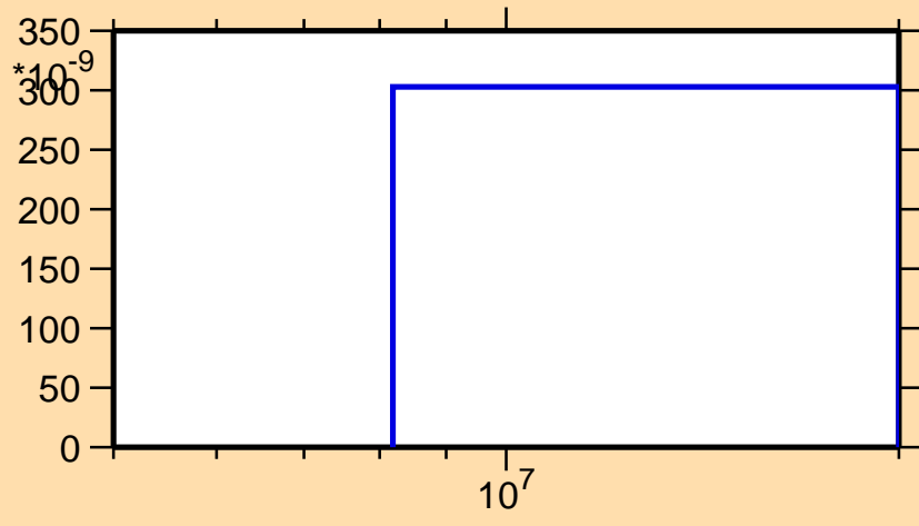
\sigma vs. E for ^{241}\text{Np}(n,2n\alpha)
