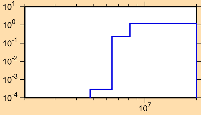
\sigma vs. E for ^{241}\text{Np}(n,2n)
