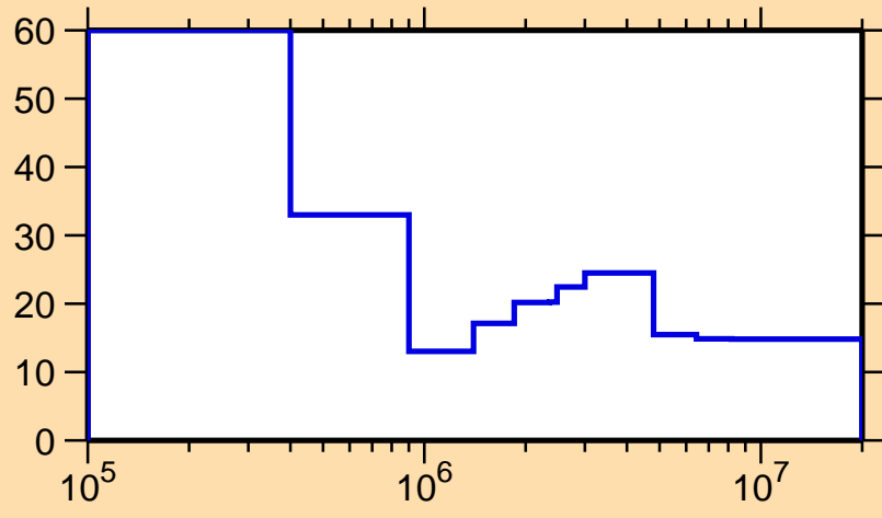
\Delta\sigma/\sigma vs. E for ^{241}\text{Np}(n,\text{nonel.})
