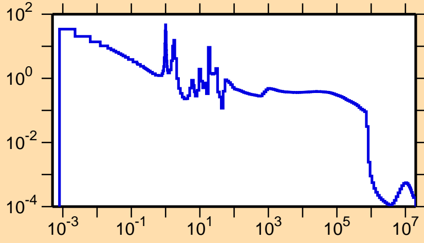
\sigma vs. E for ^{242}\text{Np}(n,\gamma)
