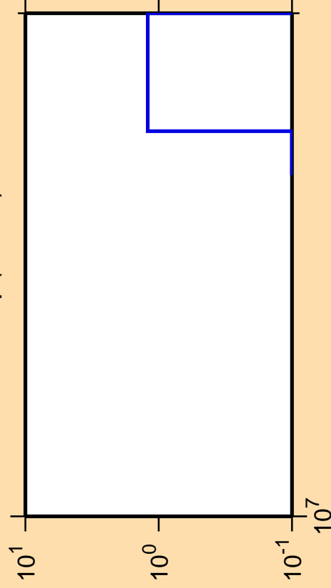
\Delta\sigma/\sigma vs. E for ^{242}\text{Np} (mt 11)
