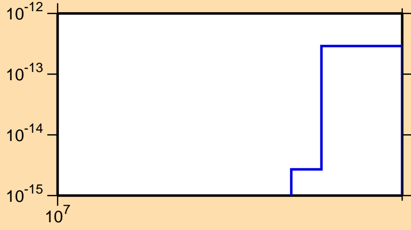
\sigma vs. E for ^{242}\text{Np}(n,\text{He3})
