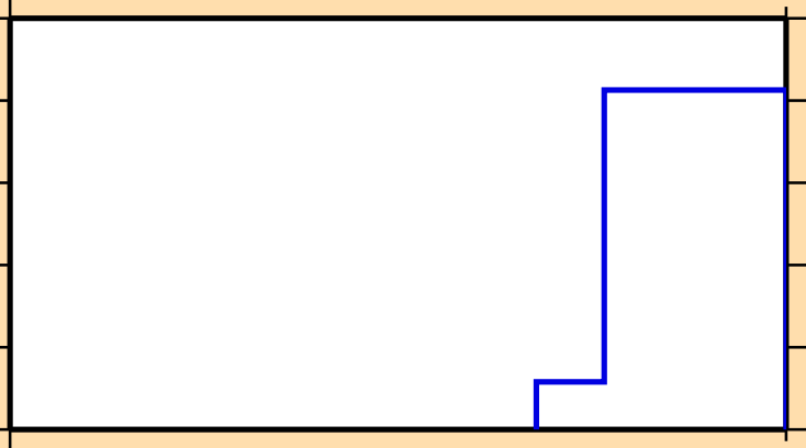
\sigma vs. E for ^{242}\text{Np} (mt 11)
