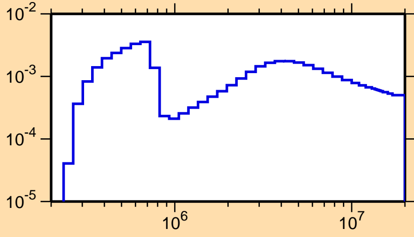
\sigma vs. E for ^{242}\text{Np}(n,n_3)
