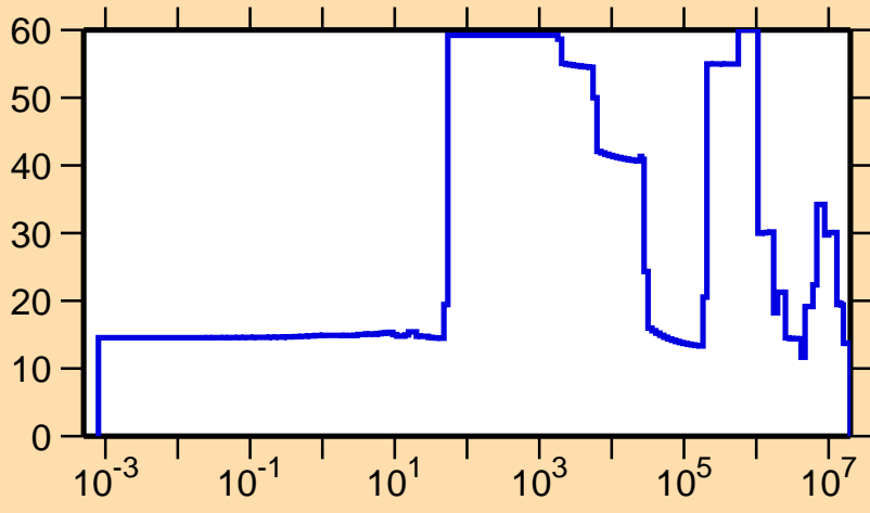
\Delta\sigma/\sigma vs. E for ^{242}\text{Np}(n,el.)
