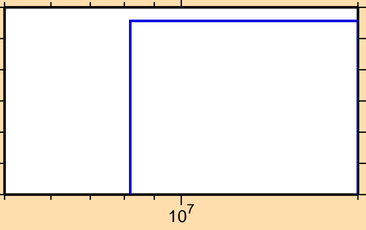
\sigma vs. E for ^{242}\text{Np}(n,2np)
