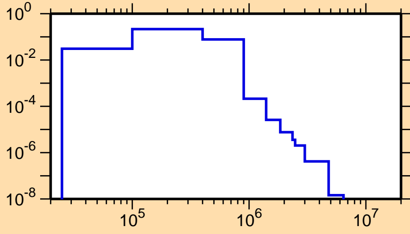
\sigma vs. E for ^{242}\text{Np}(n,n_1)
