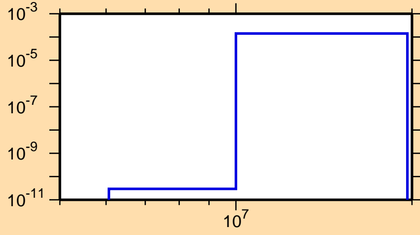
\sigma vs. E for ^{242}\text{Np}(n,d)
