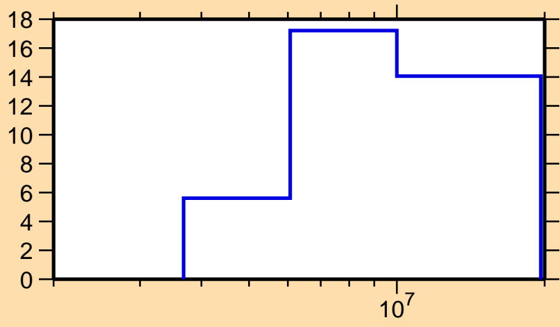
\Delta\sigma/\sigma vs. E for ^{242}\text{Np}(n,\text{tot.})
