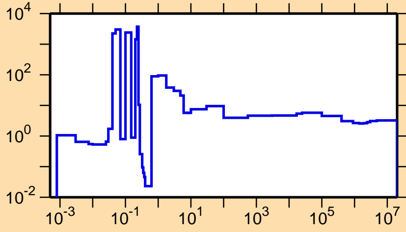
\sigma vs. E for ^{242}\text{Np}(n,\text{nonel.})
