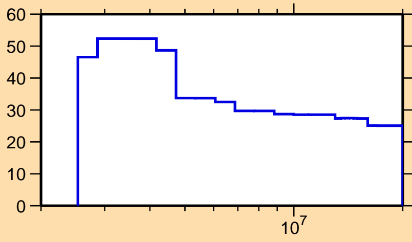
\Delta\sigma/\sigma vs. E for ^{243}\text{Np}(n,\text{nonel.})
