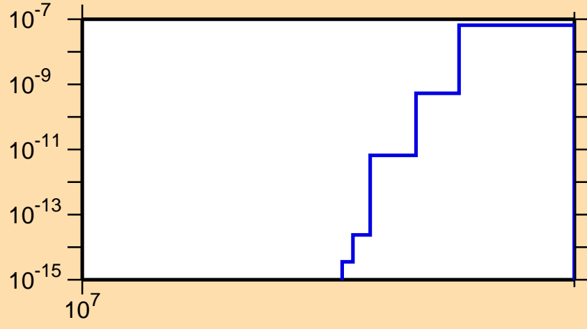
\sigma vs. E for ^{243}\text{Np}(n,2np)
