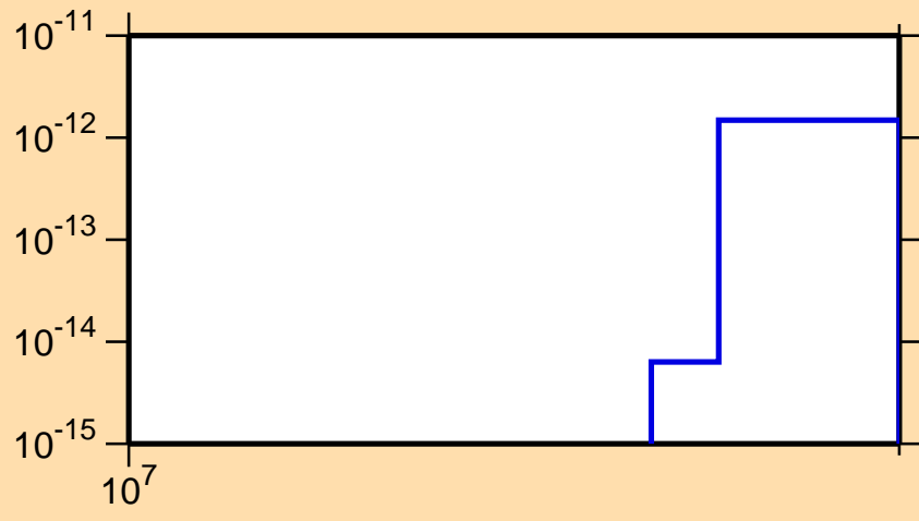
\sigma vs. E for ^{243}\text{Np}(n,\text{He3})
