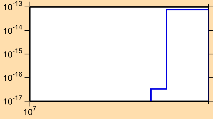
\sigma vs. E for ^{243}\text{Np} (mt 11)
