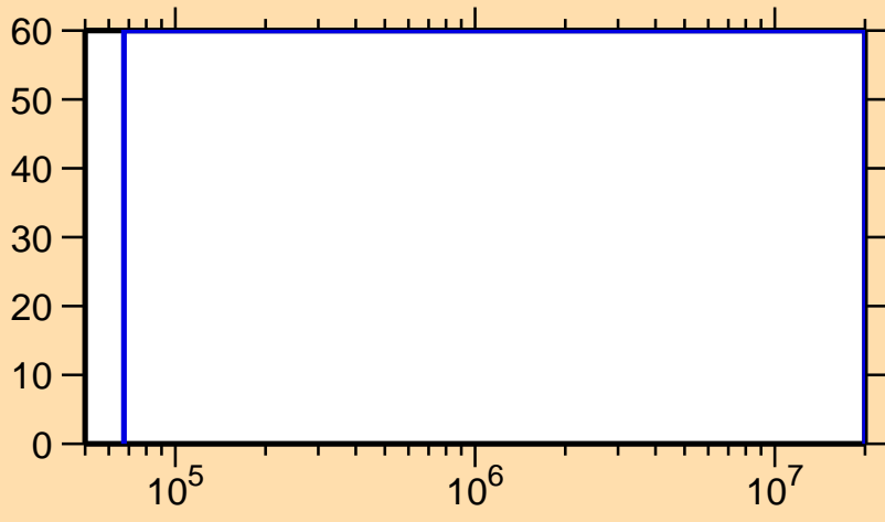
\Delta\sigma/\sigma vs. E for ^{243}\text{Np}(n,f)
