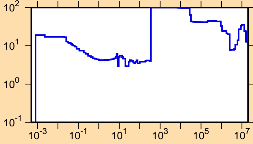
\Delta\sigma/\sigma vs. E for ^{243}\text{Np}(n,tot.)
