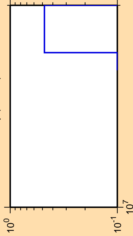
\Delta\sigma/\sigma vs. E for ^{243}\text{Np} (mt 11)
