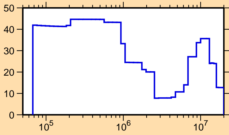
\Delta\sigma/\sigma vs. E for ^{243}\text{Np}(n,\text{tot.})
