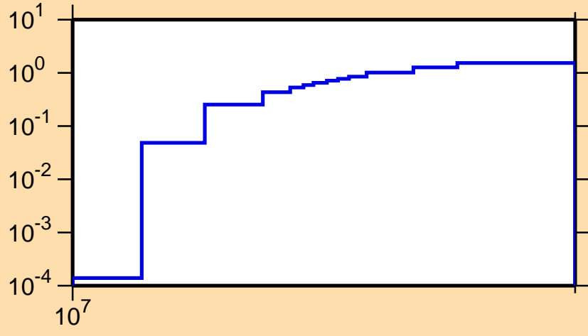
\sigma vs. E for ^{243}\text{Np}(n,3n)
