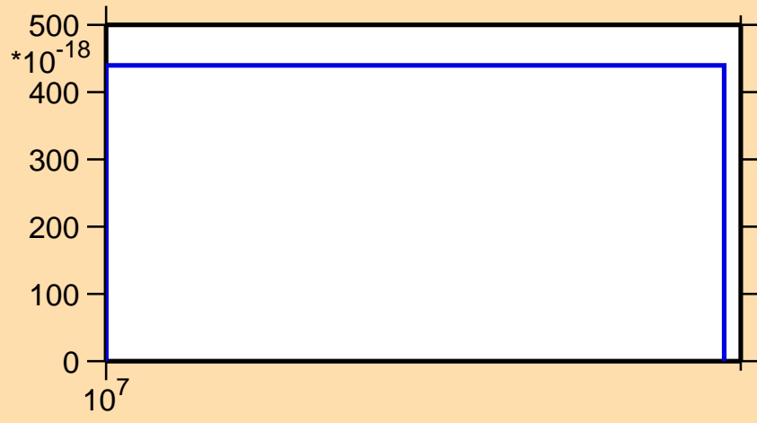
\sigma vs. E for ^{243}\text{Np} (mt 11)
