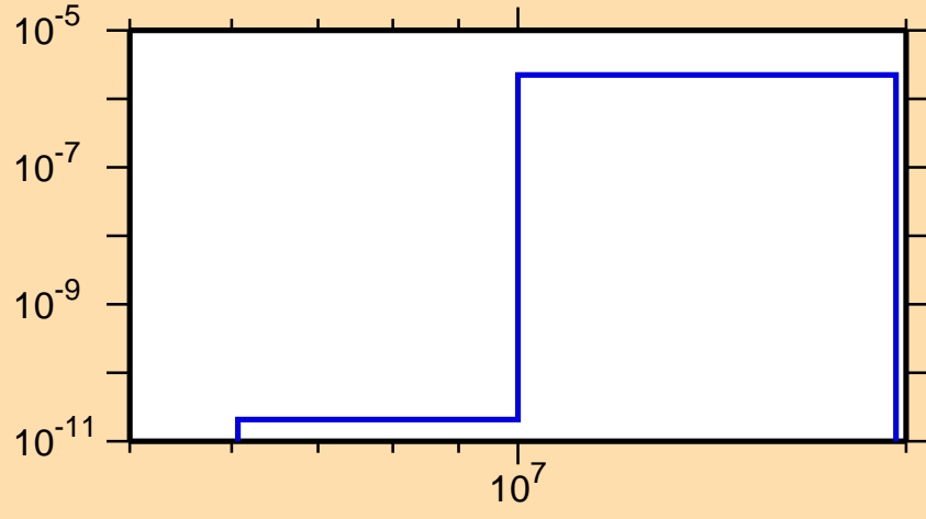
\sigma vs. E for ^{243}\text{Np}(n,n\alpha)
