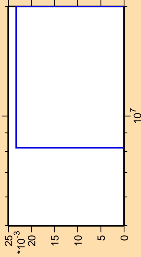
\Delta\sigma/\sigma vs. E for ^{243}\text{Np}(n,3n\alpha)
