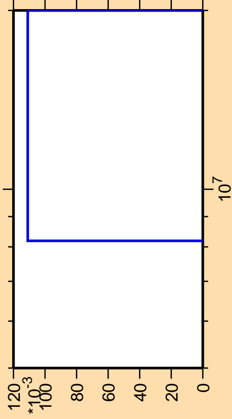
\Delta\sigma/\sigma vs. E for ^{243}\text{Np}(n,\text{He3})
