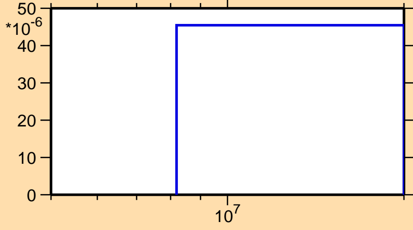
\sigma vs. E for ^{243}\text{Np}(n,t)
