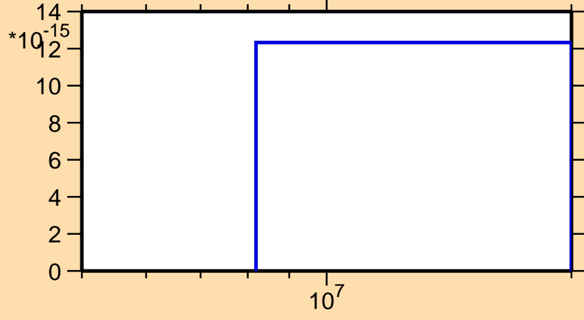
\sigma vs. E for ^{243}\text{Np}(n,\text{He3})
