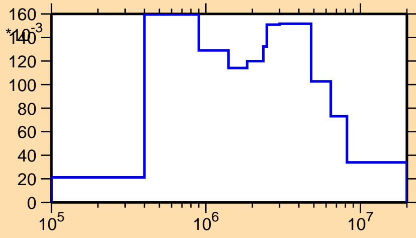
\sigma vs. E for ^{243}\text{Np}(n,n_4)
