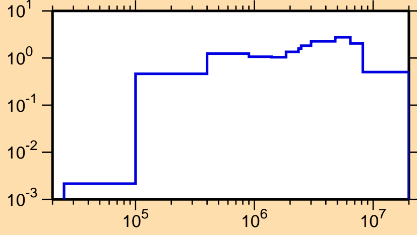
\sigma vs. E for ^{243}\text{Np}(n,\text{inel.})
