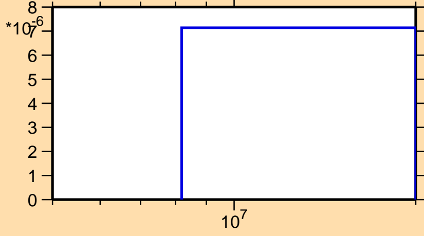
\sigma vs. E for ^{243}\text{Np}(n,np)
