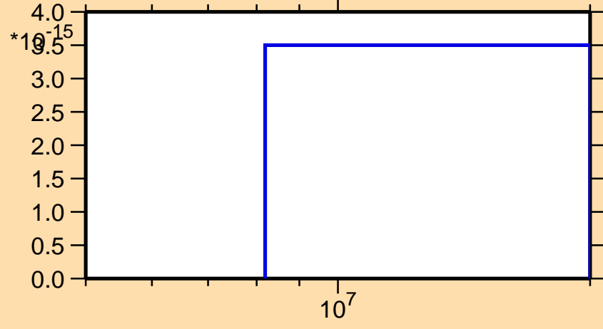
\sigma vs. E for ^{243}\text{Np}(n,3n\alpha)
