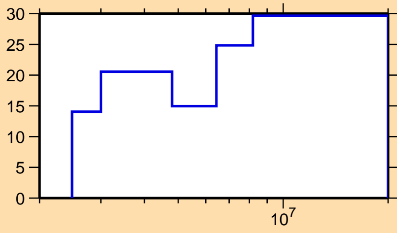
\Delta\sigma/\sigma vs. E for ^{243}\text{Np}(n,\text{el.})
