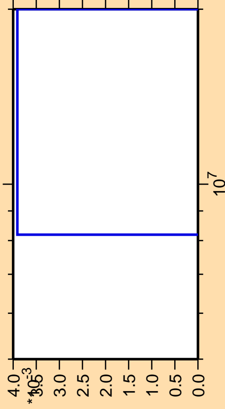
\Delta\sigma/\sigma vs. E for ^{243}\text{Np}(\text{mt } 11)
