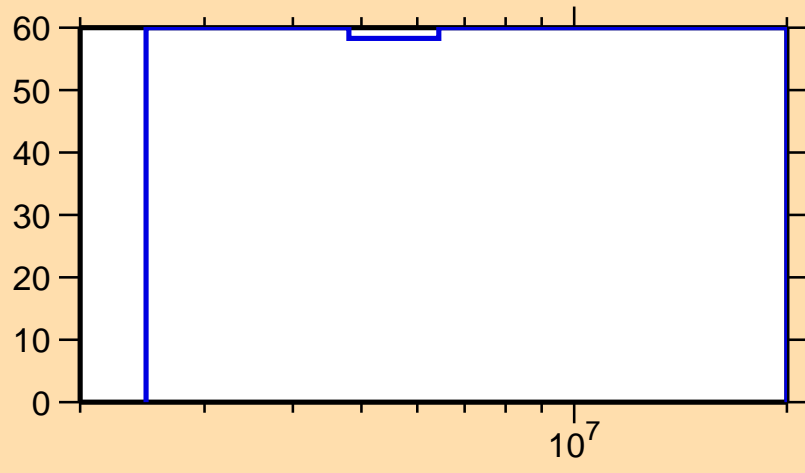
\Delta\sigma/\sigma vs. E for ^{243}\text{Np}(n,n\text{cont.})
