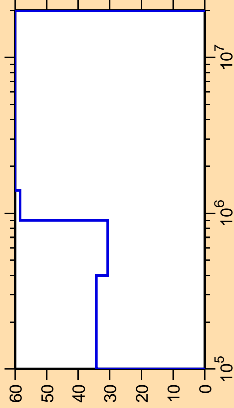
\Delta\sigma/\sigma vs. E for ^{243}\text{Np}(n,n_4)
