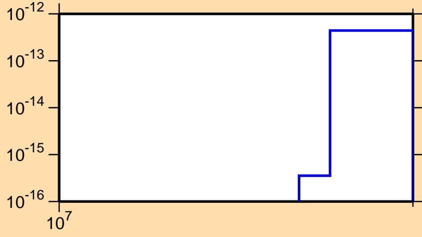
\sigma vs. E for ^{244}\text{Np} (mt 11)
