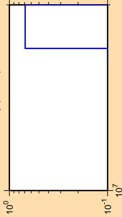
\Delta\sigma/\sigma vs. E for ^{244}\text{Np} (mt 11)
