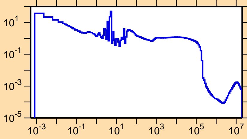
\sigma vs. E for ^{244}\text{Np}(n,\gamma)
