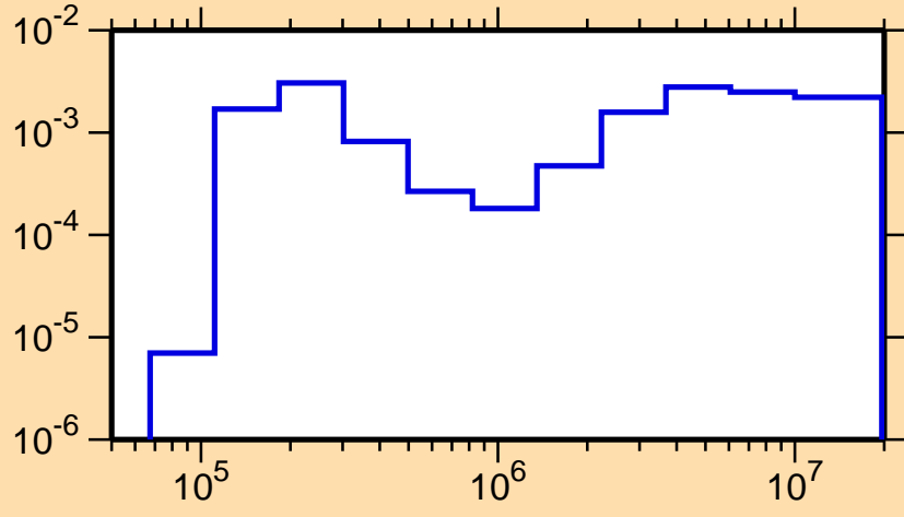
\sigma vs. E for ^{244}\text{Np}(n,n_1)
