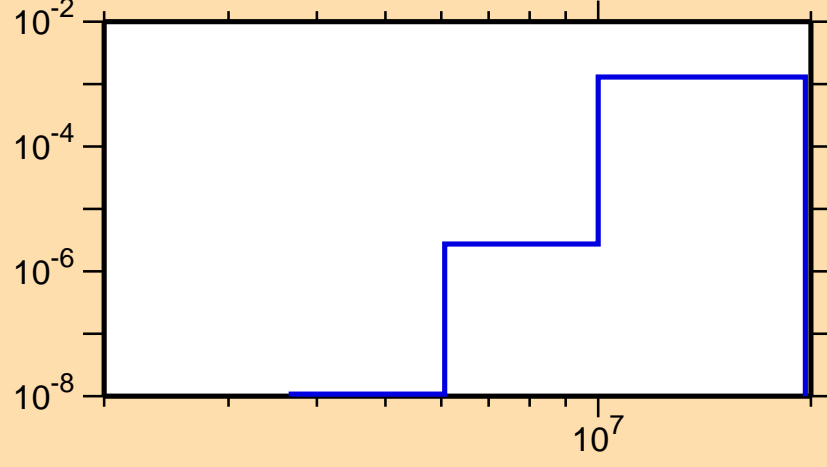
\sigma vs. E for ^{244}\text{Np}(n,\alpha)
