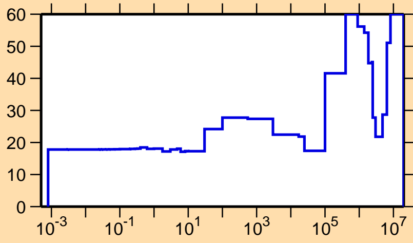
\Delta\sigma/\sigma vs. E for ^{244}\text{Np}(n,el.)
