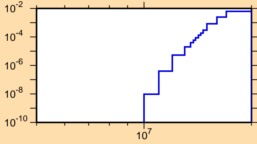
\sigma vs. E for ^{245}\text{Np}(n,np)
