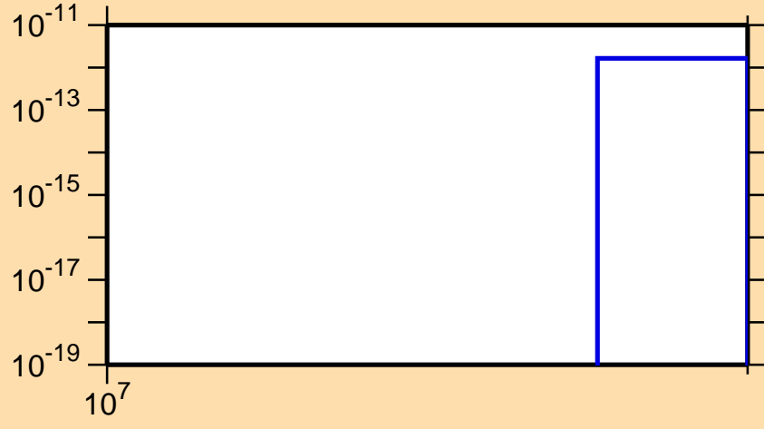
\sigma vs. E for ^{245}\text{Np} (mt 11)
