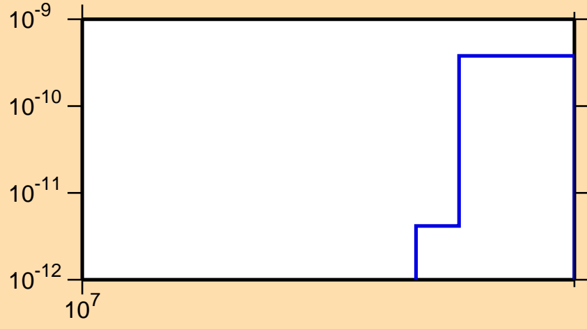
\sigma vs. E for ^{245}\text{Np}(n,3n\alpha)
