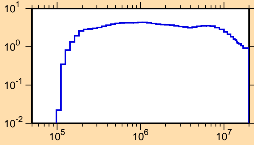
\sigma vs. E for ^{245}\text{Np}(n,\text{inel.})
