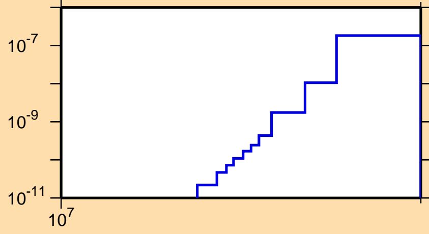
\sigma vs. E for ^{245}\text{Np}(n,2n\alpha)
