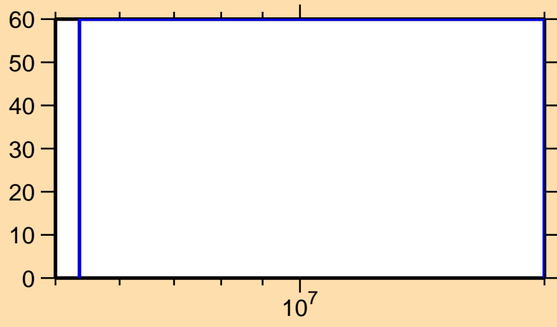
\Delta\sigma/\sigma vs. E for ^{245}\text{Np}(n,\text{inel.})
