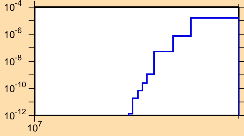
\sigma vs. E for ^{245}\text{Np}(n,\text{nd})
