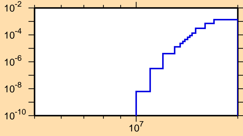
\sigma vs. E for ^{245}\text{Np}(n,t)
