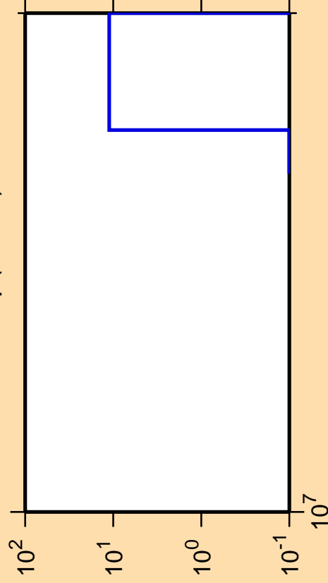
\Delta\sigma/\sigma vs. E for ^{245}\text{Np} (mt 11)
