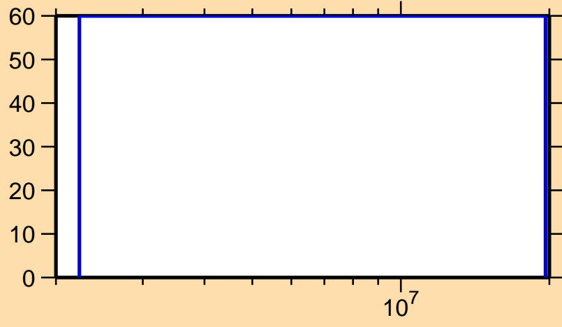
\Delta\sigma/\sigma vs. E for ^{245}\text{Np}(n,n\text{cont.})
