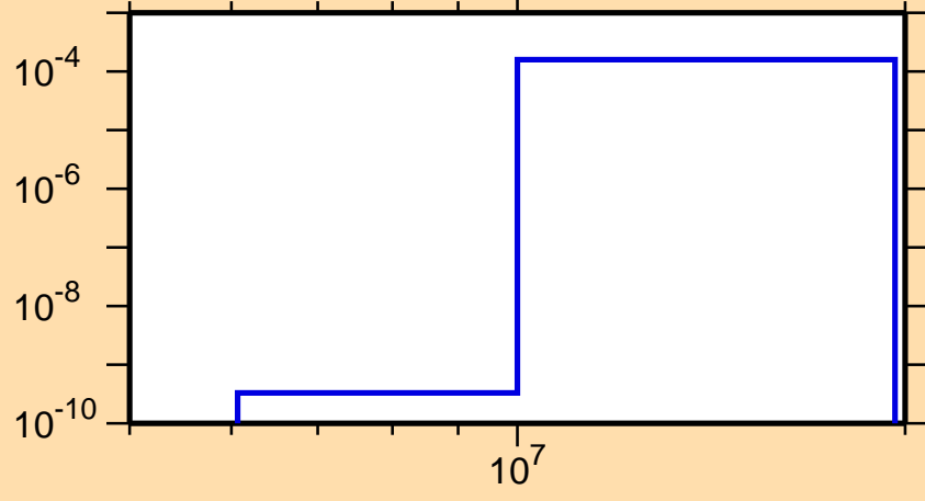
\sigma vs. E for ^{245}\text{Np}(n,n\alpha)
