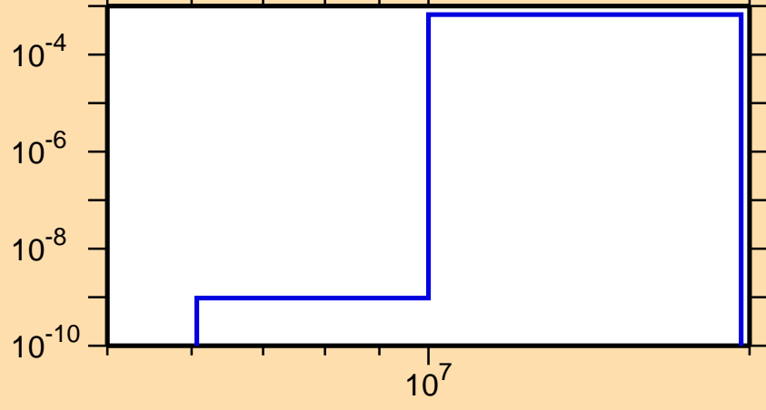
\sigma vs. E for ^{245}\text{Np}(n,d)
