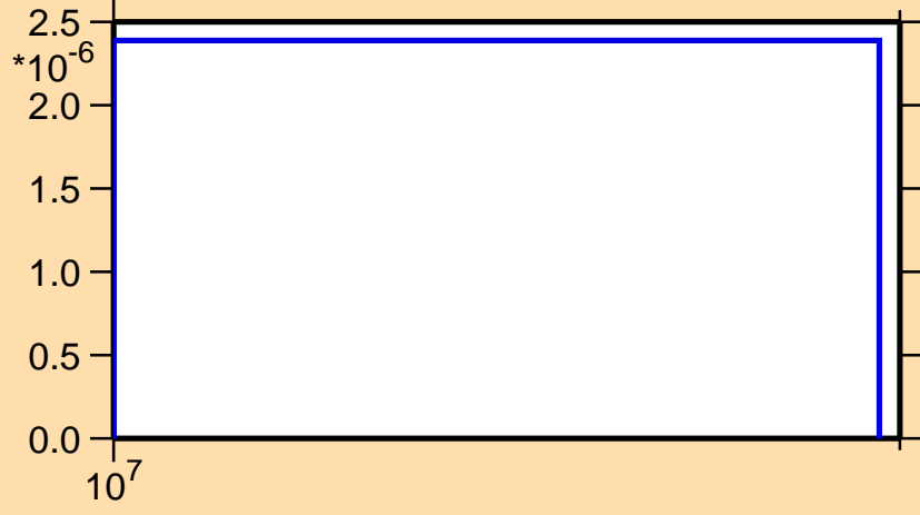
\sigma vs. E for ^{245}\text{Np}(n,nt)
