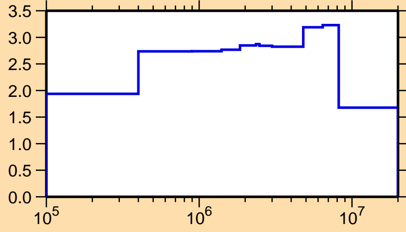
\sigma vs. E for ^{245}\text{Np}(n,n\text{cont.})
