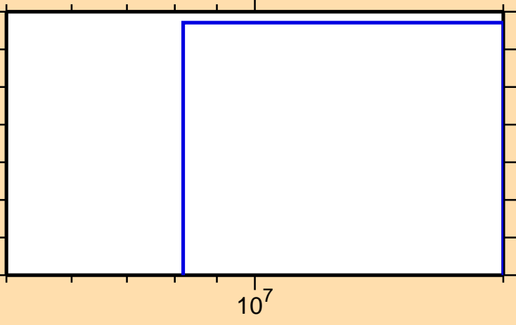
\sigma vs. E for ^{245}\text{Np}(\text{mt } 11)
