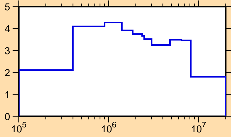
\sigma vs. E for ^{245}\text{Np}(n,\text{inel.})
