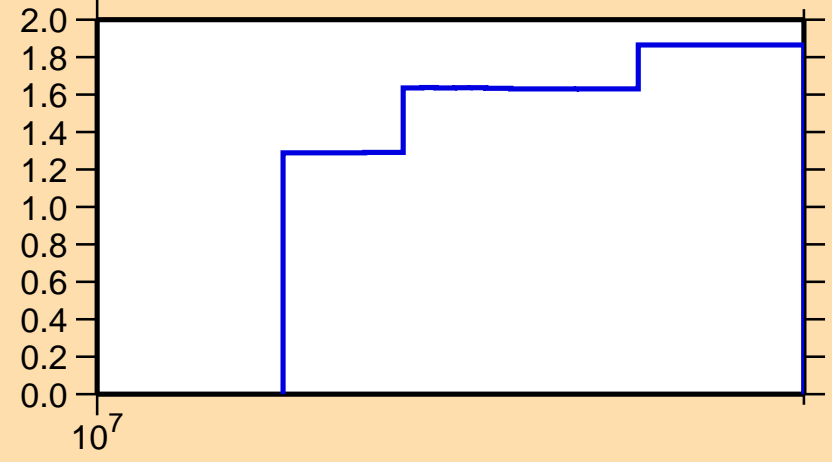
\Delta\sigma/\sigma vs. E for ^{20}\text{O}(n,\text{nonel.})
