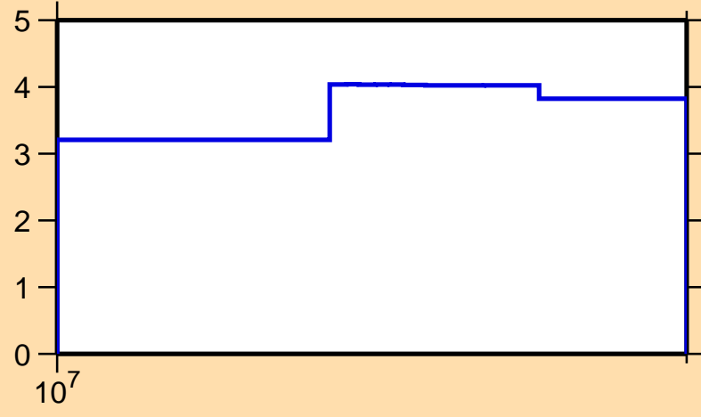
\Delta\sigma/\sigma vs. E for ^{20}\text{O}(n,2n)
