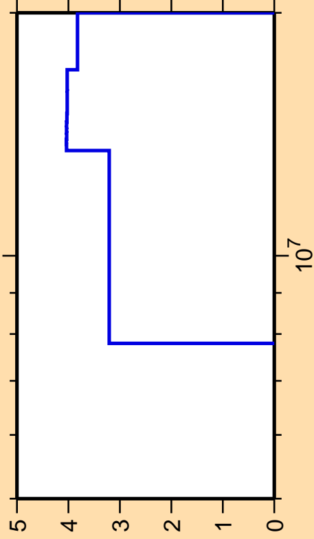
\Delta\sigma/\sigma vs. E for ^{20}\text{O}(n,2n)
