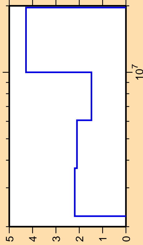
\Delta\sigma/\sigma vs. E for ^{20}\text{O}(n,\text{inel.})
