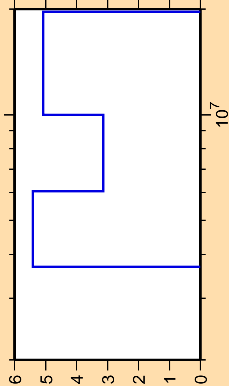
\Delta\sigma/\sigma vs. E for ^{20}\text{O}(n,n_2)
