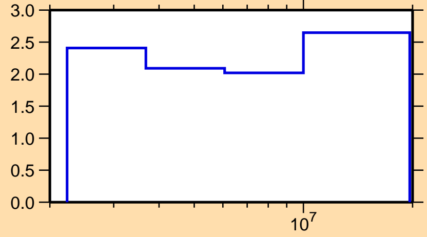
\Delta\sigma/\sigma vs. E for ^{20}\text{O}(n,\text{el.})
