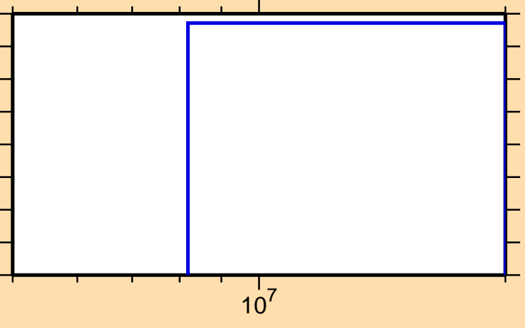
\sigma vs. E for ^{20}\text{O}(n,3n\alpha)
