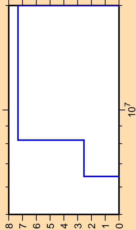
\Delta\sigma/\sigma vs. E for ^{20}\text{O}(n,n_1)
