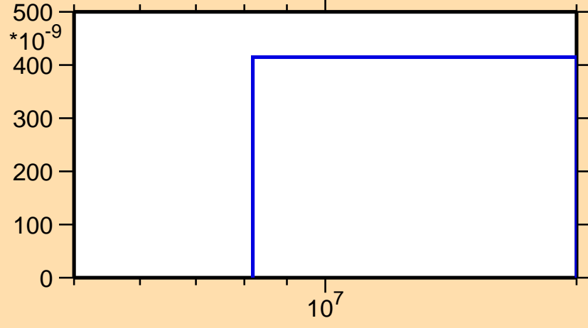
\sigma vs. E for ^{20}\text{O}(n,t)
