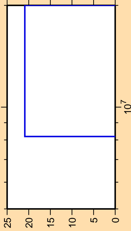
\Delta\sigma/\sigma vs. E for ^{20}\text{O}(n,d)
