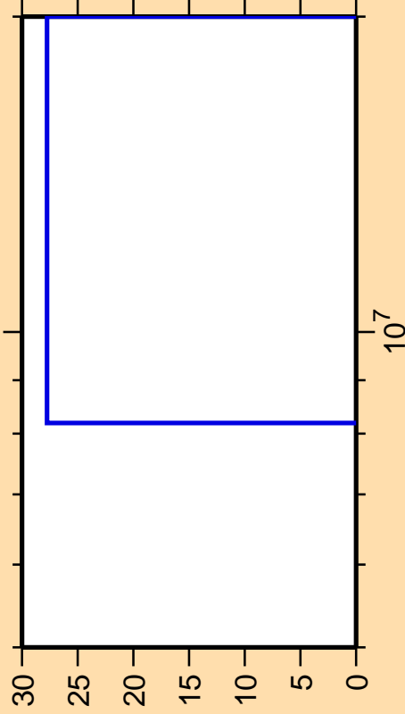
\Delta\sigma/\sigma vs. E for ^{20}\text{O}(n,p)
