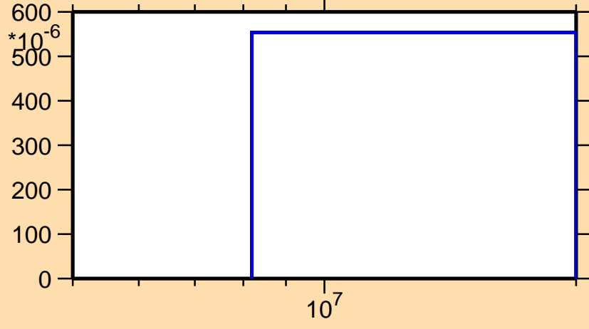
\sigma vs. E for ^{20}\text{O}(n,\alpha)
