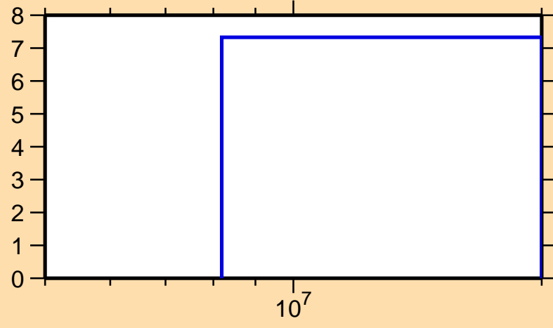
\Delta\sigma/\sigma vs. E for ^{20}\text{O}(n,n_1)
