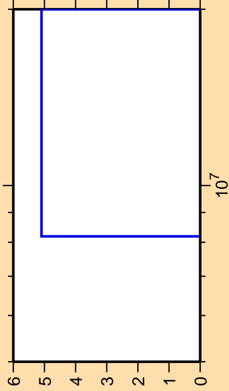
\Delta\sigma/\sigma vs. E for ^{20}\text{O}(n,3n)
