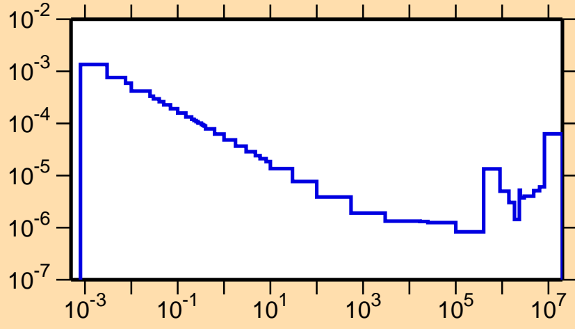
\sigma vs. E for ^{20}\text{O}(n,\gamma)
