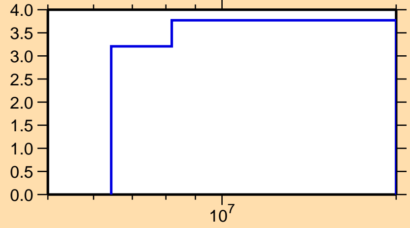
\Delta\sigma/\sigma vs. E for ^{20}\text{O}(n,2n)
