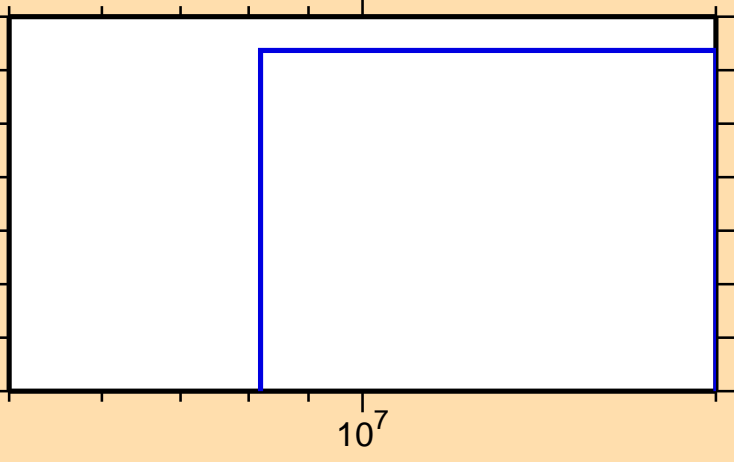
\sigma vs. E for ^{20}\text{O}(n,d)
