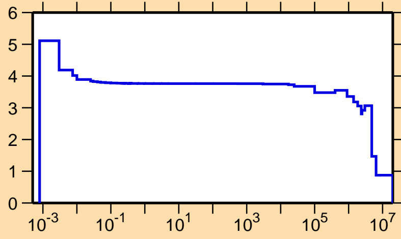
\sigma vs. E for ^{22}\text{O}(n,\text{el.})
