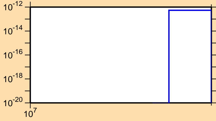
\sigma vs. E for ^{168}\text{Os}(n,nt)
