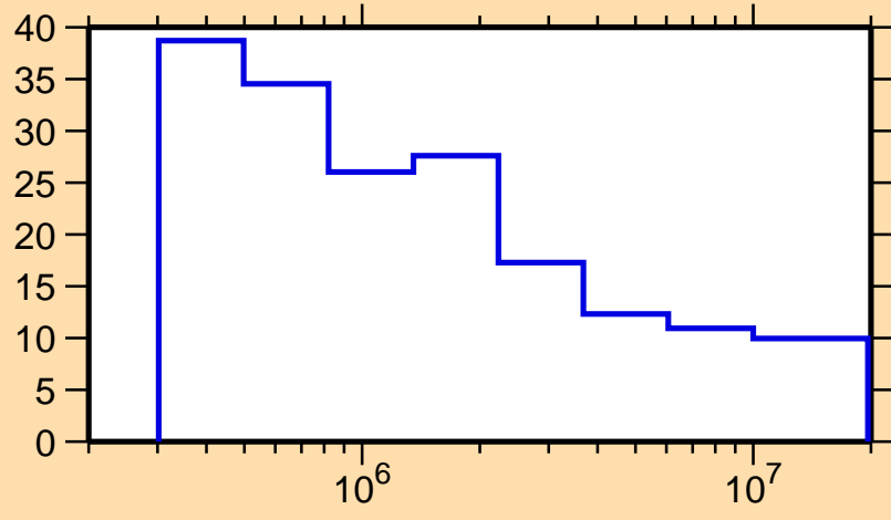
\Delta\sigma/\sigma vs. E for ^{168}\text{Os}(n,\text{nonel.})
