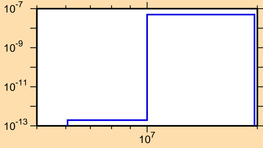
\sigma vs. E for ^{168}\text{Os}(\text{mt117})
