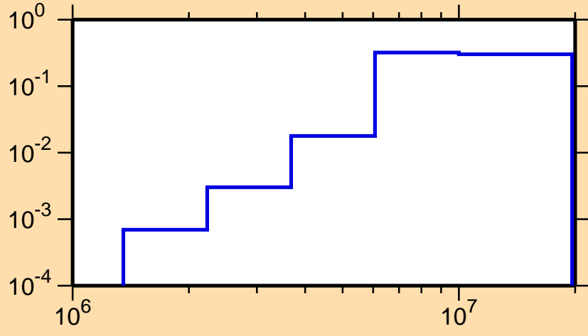
\sigma vs. E for ^{168}\text{Os}(n,n\text{cont.})
