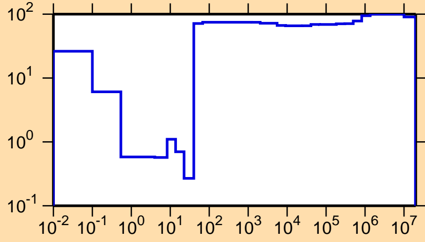
\Delta\sigma/\sigma vs. E for ^{168}\text{Os}(n,\gamma)
