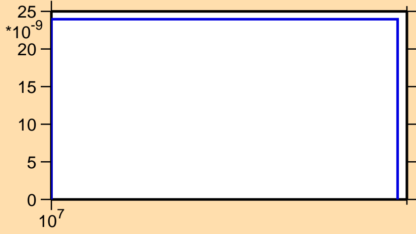
\sigma vs. E for ^{168}\text{Os}(n,\text{pt})
