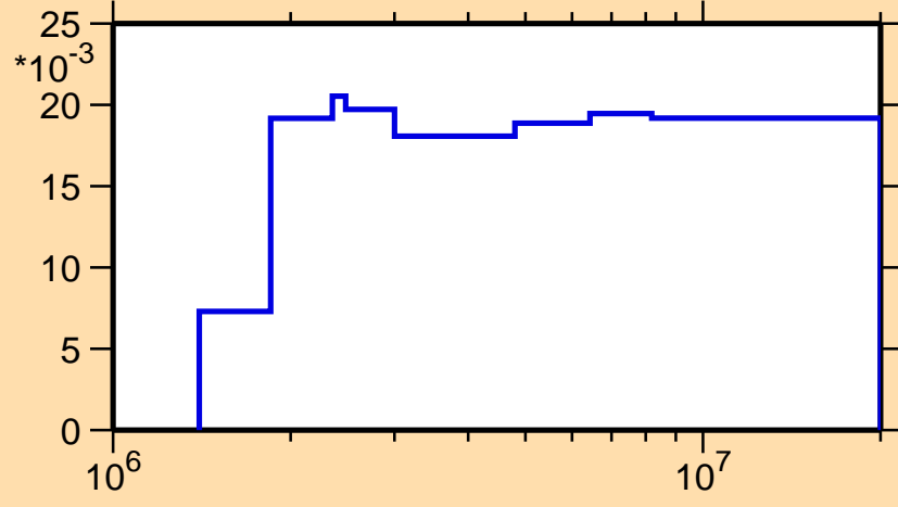
\sigma vs. E for ^{168}\text{Os}(n,n_3)
