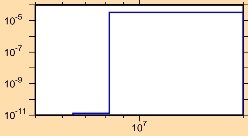
\sigma vs. E for ^{168}\text{Os} (mt 45)
