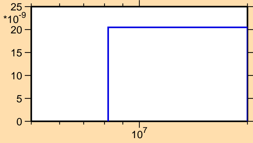
\sigma vs. E for ^{168}\text{Os}(n,pt)
