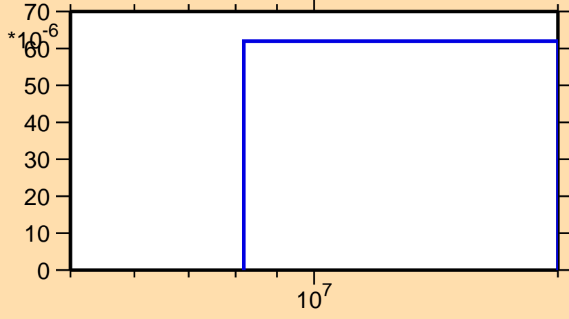
\sigma vs. E for ^{168}\text{Os}(n,t)
