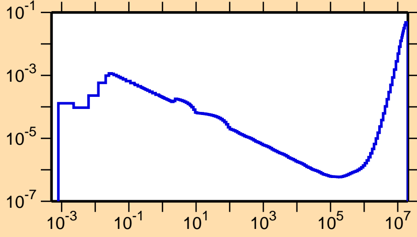
\sigma vs. E for ^{169}\text{Os}(n,p\alpha)
