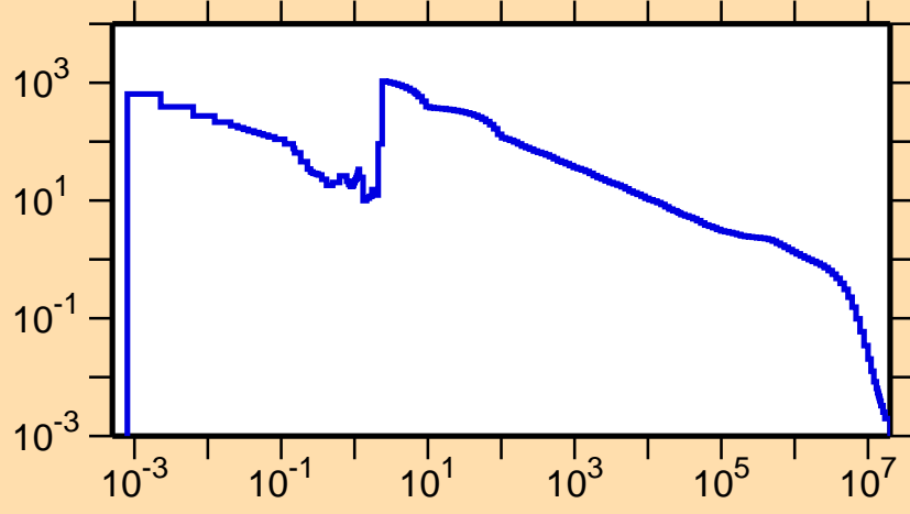
\sigma vs. E for ^{169}\text{Os}(n,\gamma)
