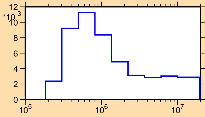
\sigma vs. E for ^{169}\text{Os}(n,n_4)
