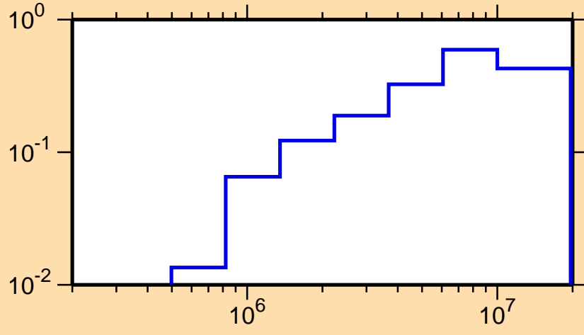
\sigma vs. E for ^{169}\text{Os}(n,n\text{cont.})
