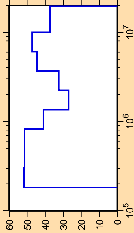
\Delta\sigma/\sigma vs. E for ^{169}\text{Os}(n,n_4)
