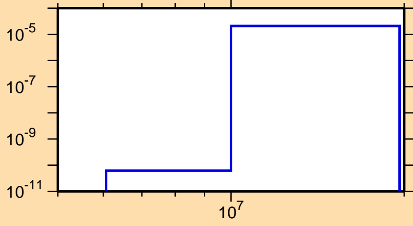
\sigma vs. E for ^{169}\text{Os}(\text{mt } 45)
