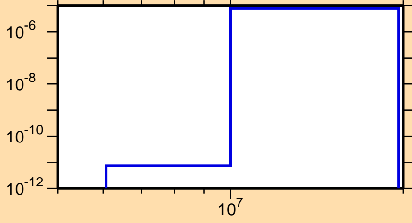
\sigma vs. E for ^{169}\text{Os}(n,pd)
