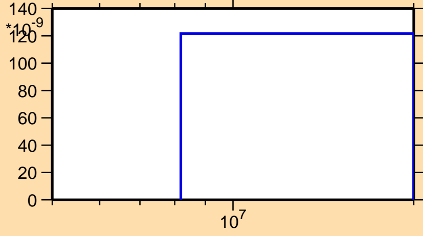
\sigma vs. E for ^{169}\text{Os}(n,\text{nd})
