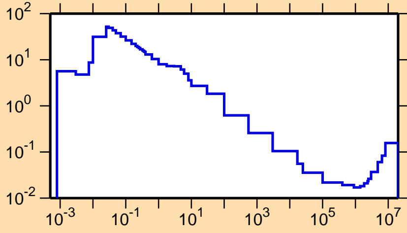
\sigma vs. E for ^{169}\text{Os}(n,\alpha)
