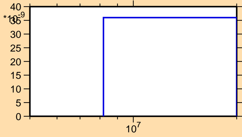
\sigma vs. E for ^{169}\text{Os}(\text{mt117})
