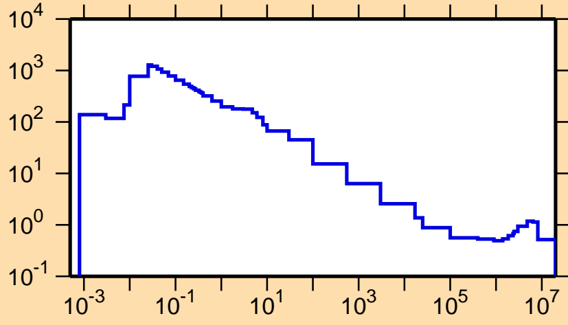
\sigma vs. E for ^{169}\text{Os}(n,p)
