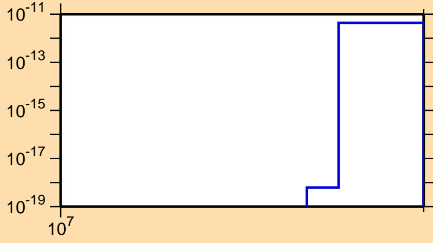
\sigma vs. E for ^{170}\text{Os}(n,nt)
