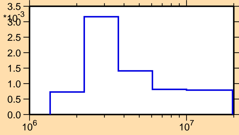
\sigma vs. E for ^{170}\text{Os}(n,n_4)
